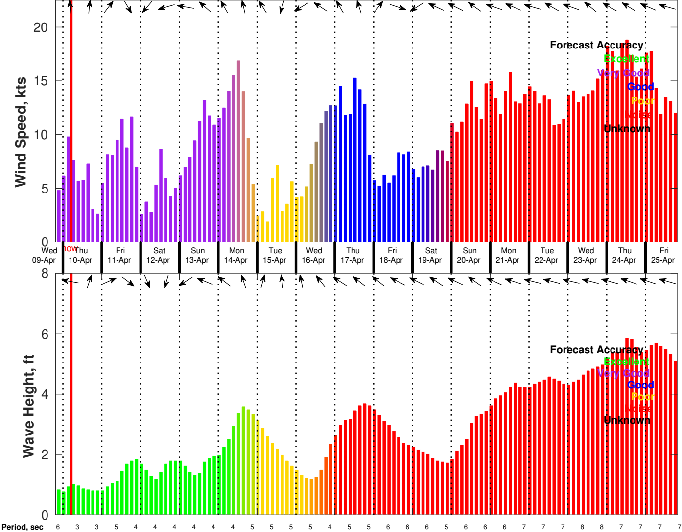
Wind & Wave Forecast for CTI Enbridge Kaskida & Tiber PPL Geotechnical from 09-Apr-2025 20:00:00 to 25-Apr-2025 20:00:00
