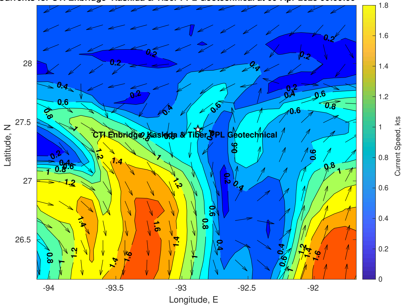
Surface Currents for CTI Enbridge Kaskida & Tiber PPL Geotechnical at 09-Apr-2025 00:00:00
