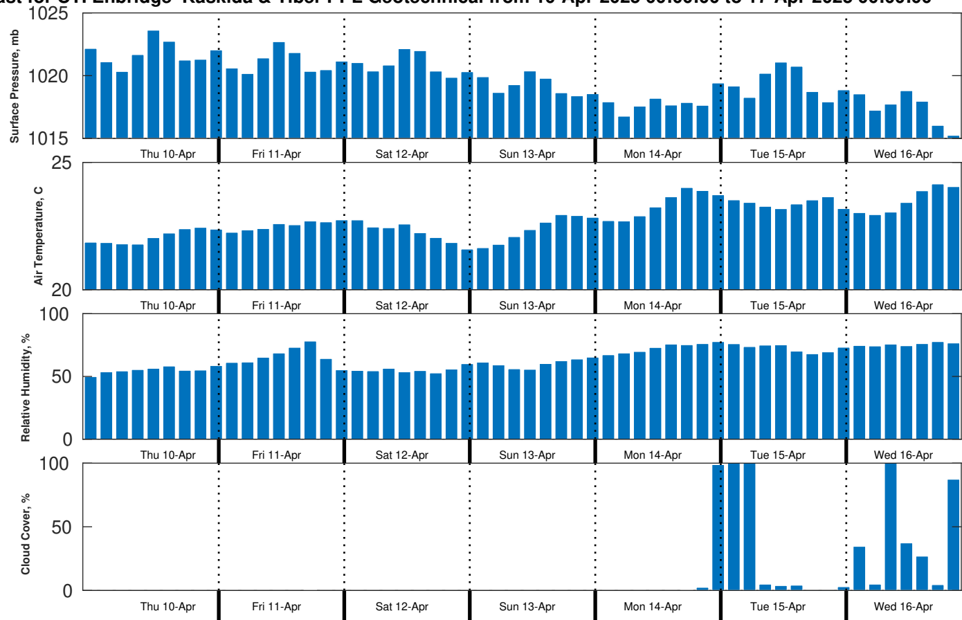
Met Forecast for CTI Enbridge Kaskida & Tiber PPL Geotechnical from 10-Apr-2025 00:00:00 to 17-Apr-2025 00:00:00
