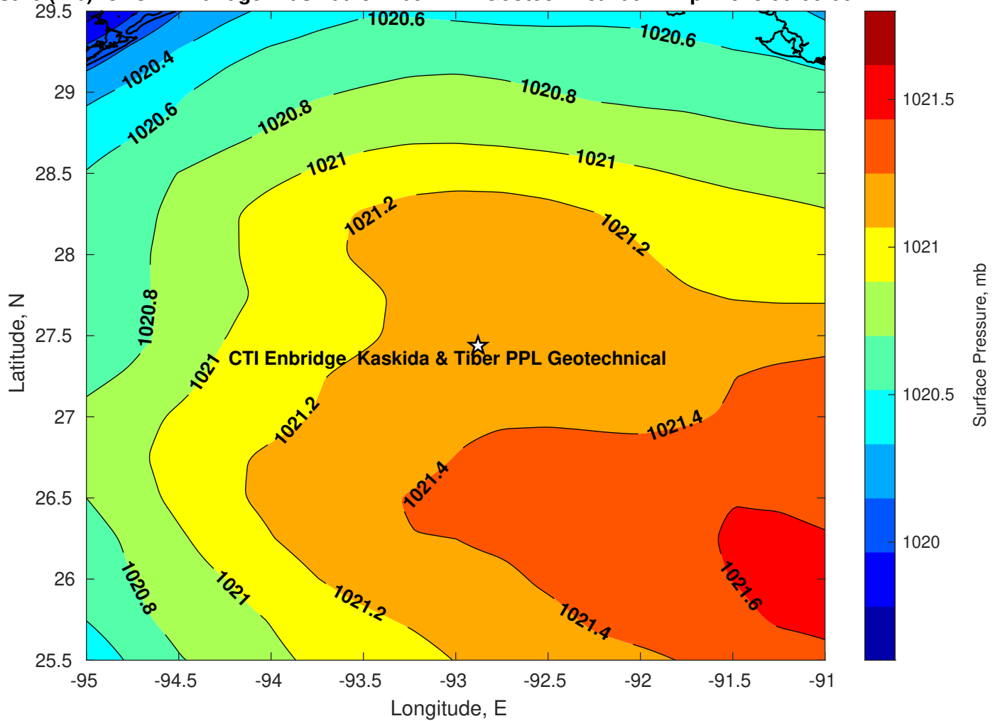
Surface Pressure (mb) for CTI Enbridge Kaskida & Tiber PPL Geotechnical at 11-Apr-2025 00:00:00
