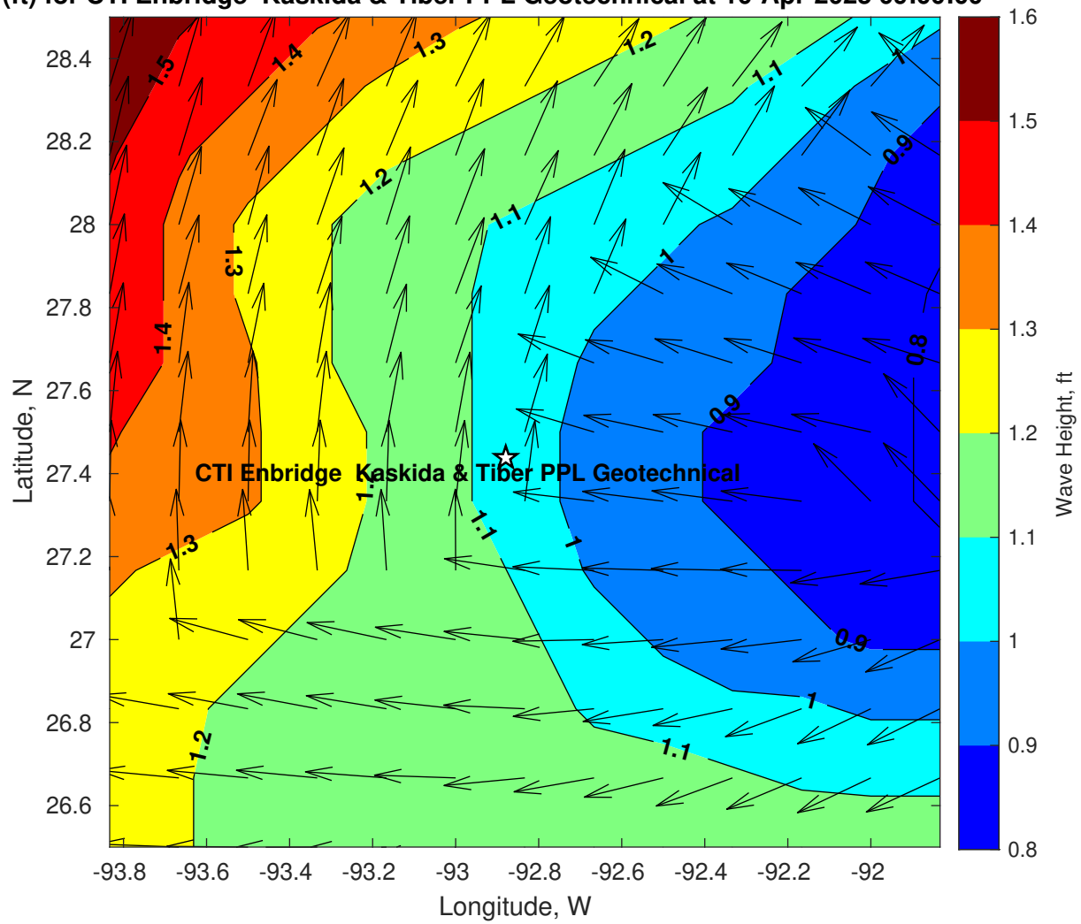
Wave Height (ft) for CTI Enbridge Kaskida & Tiber PPL Geotechnical at 10-Apr-2025 09:00:00
