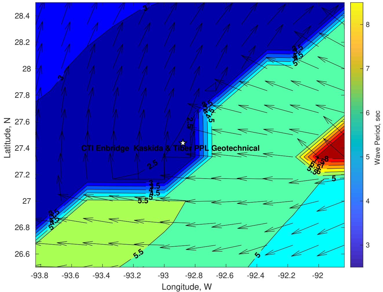
Wave Period (sec) for CTI Enbridge Kaskida & Tiber PPL Geotechnical at 10-Apr-2025 09:00:00
