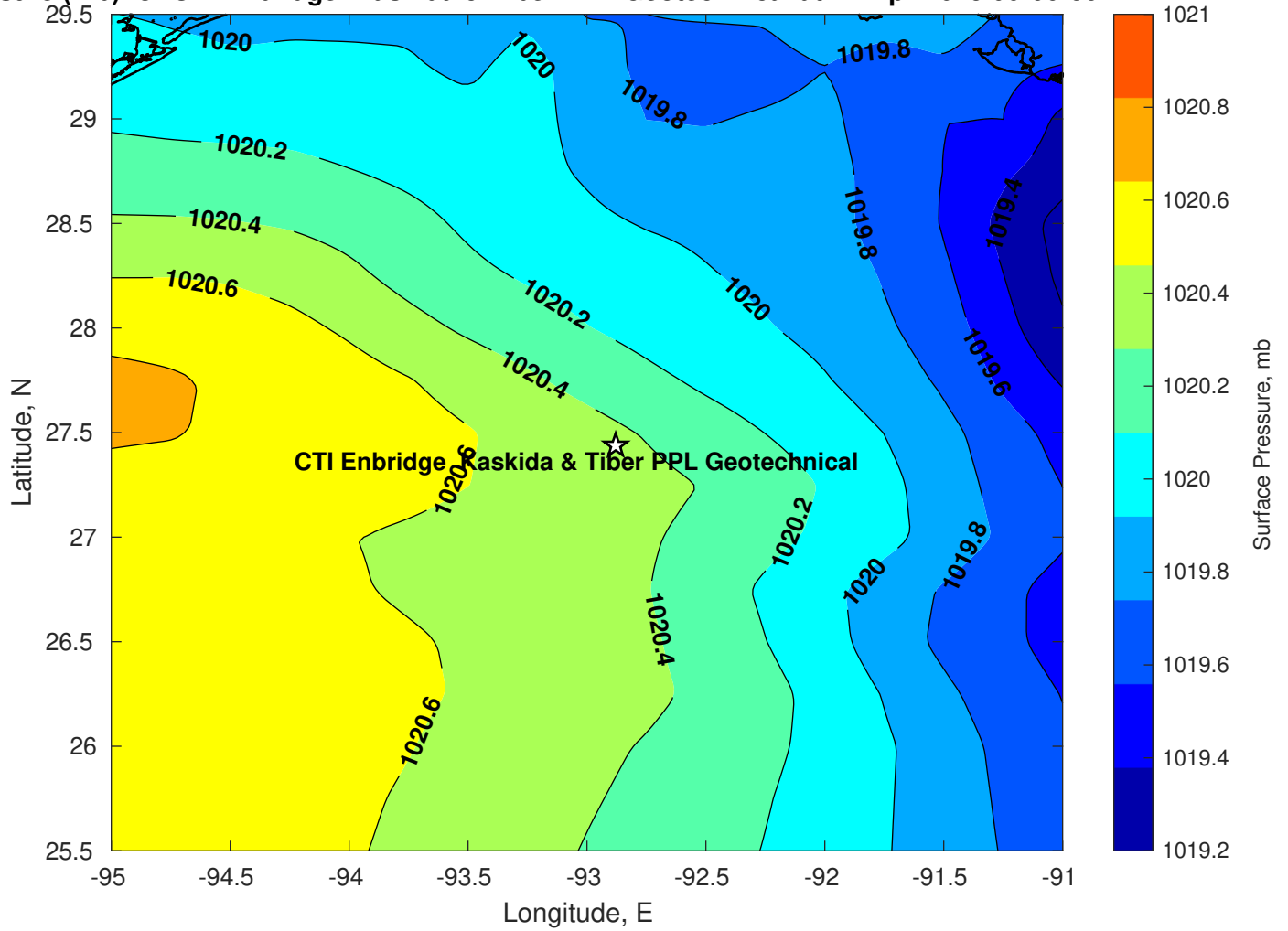
Surface Pressure (mb) for CTI Enbridge Kaskida & Tiber PPL Geotechnical at 12-Apr-2025 00:00:00
