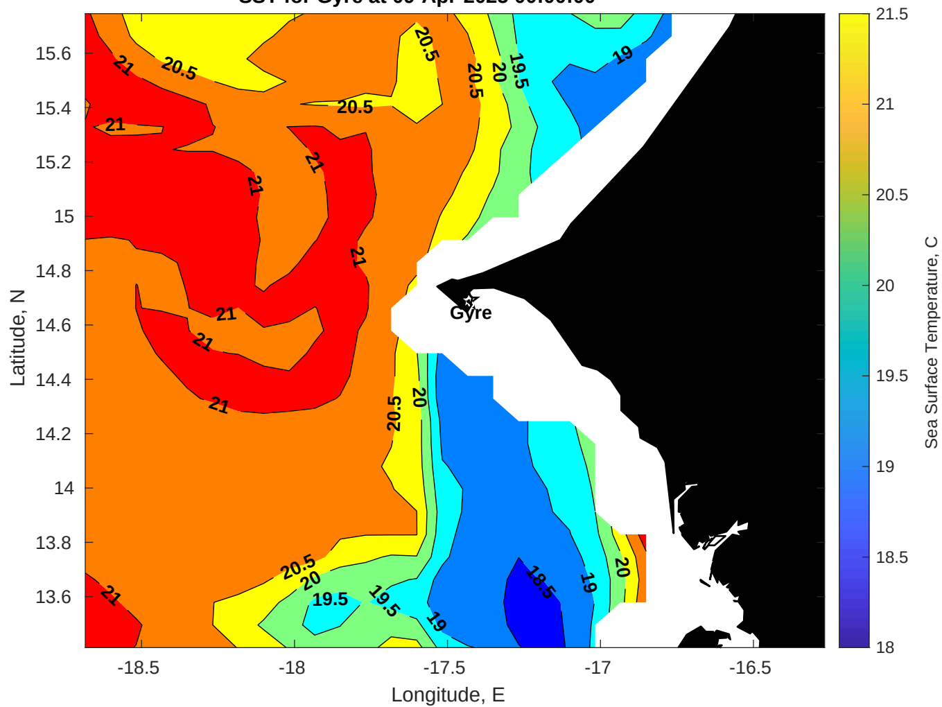
SST for Gyre at 09-Apr-2025 00:00:00
