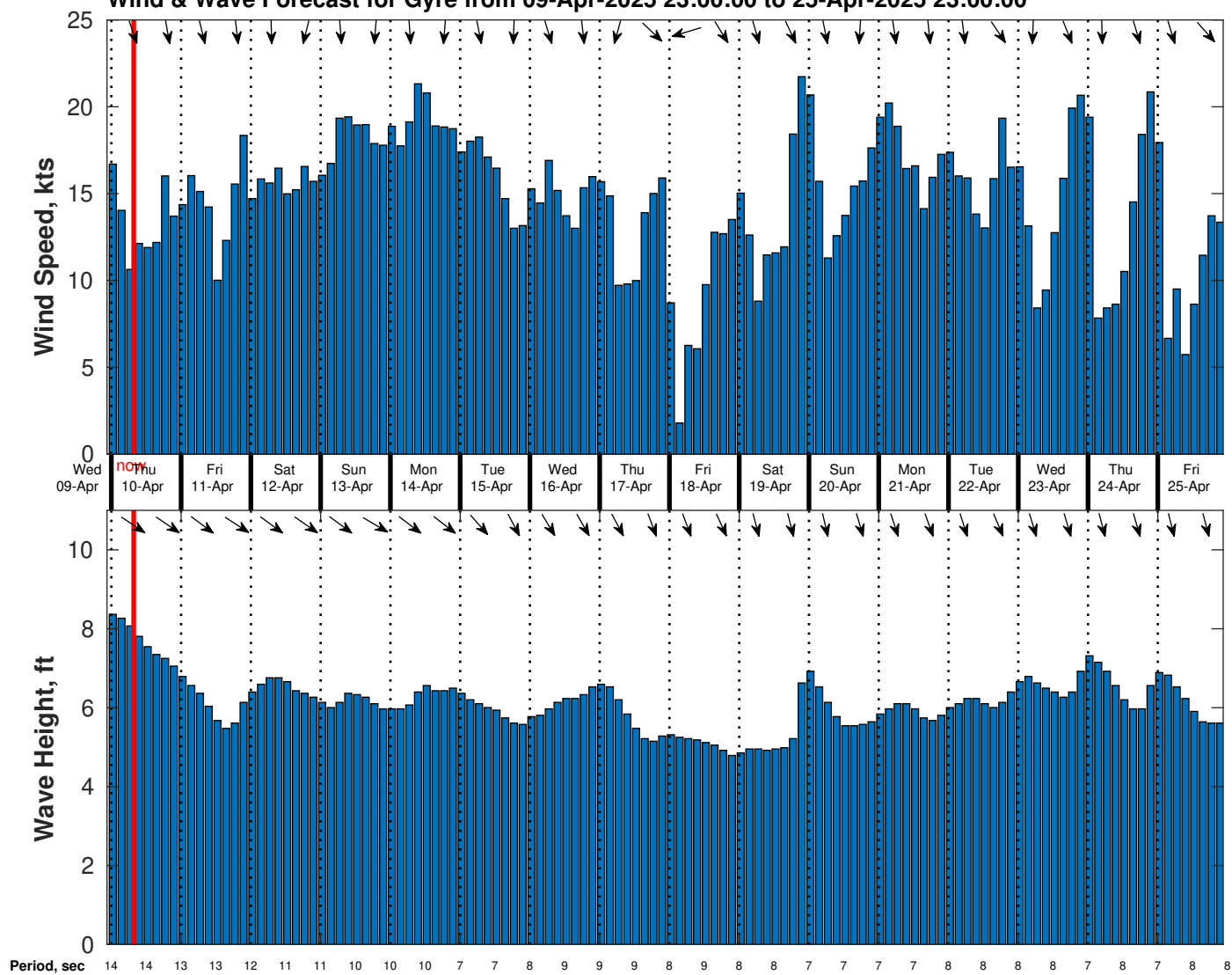
Wind & Wave Forecast for Gyre from 09-Apr-2025 23:00:00 to 25-Apr-2025 23:00:00
