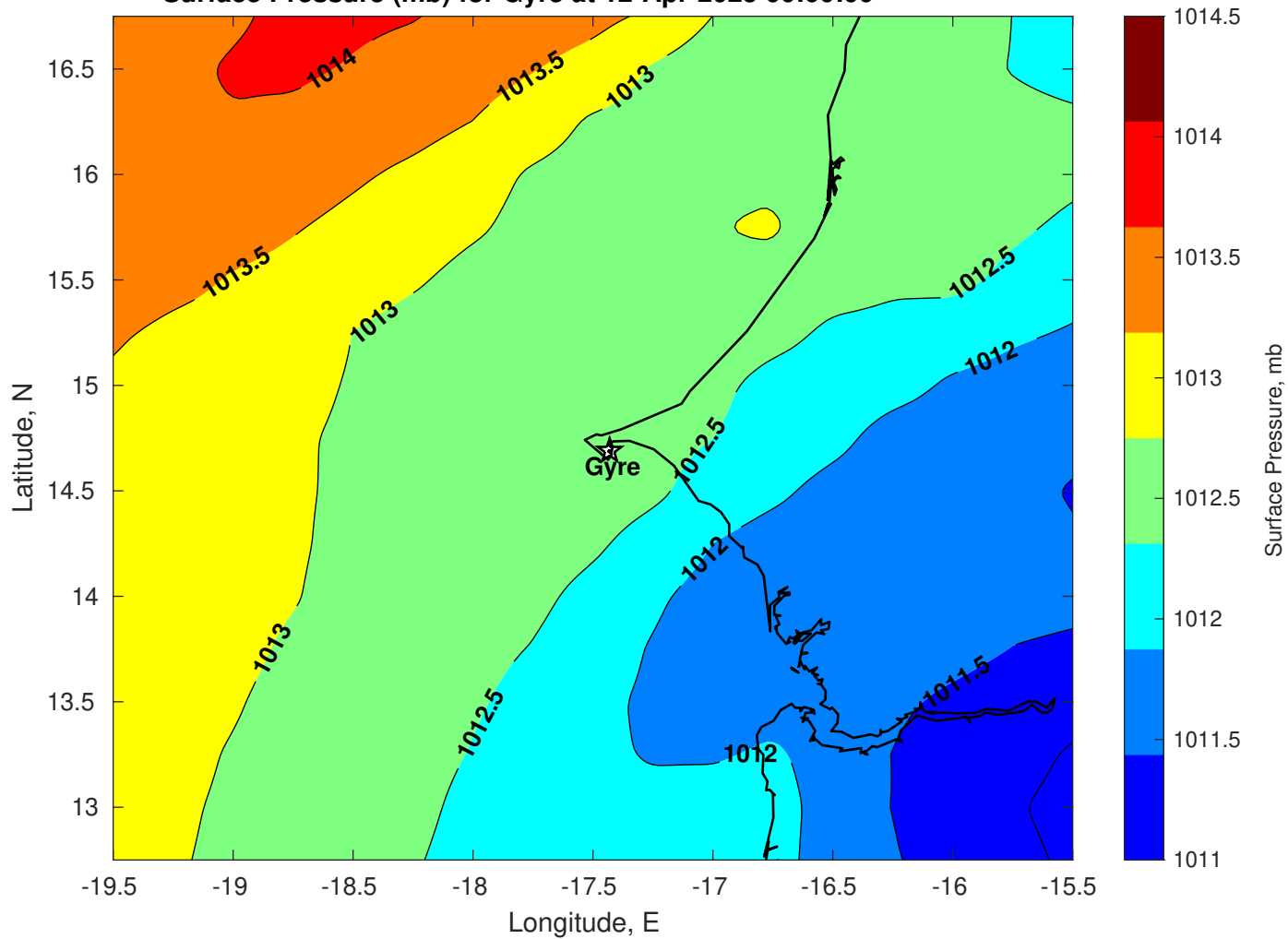
Surface Pressure (mb) for Gyre at 12-Apr-2025 00:00:00
