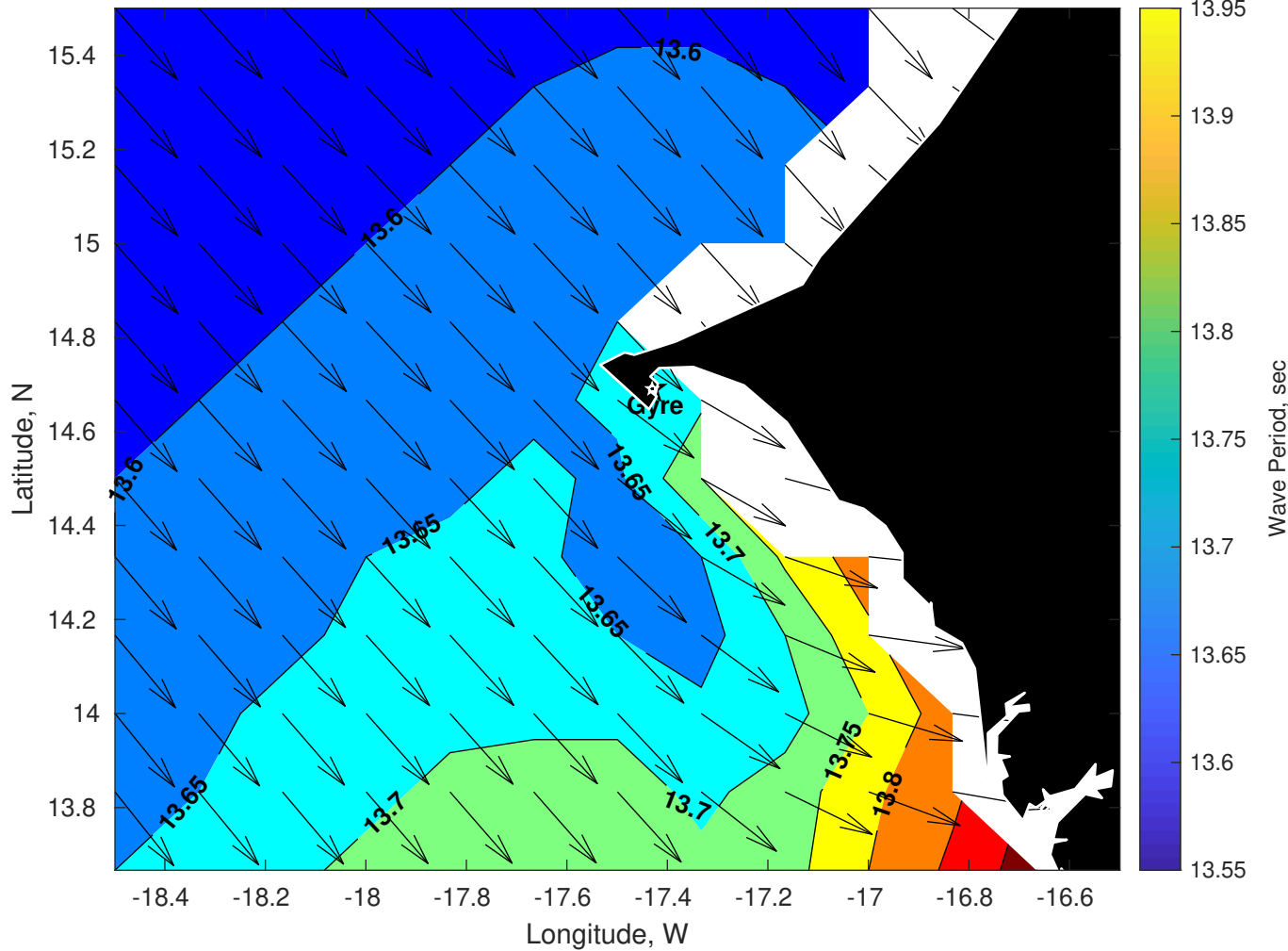
Wave Period (sec) for Gyre at 10-Apr-2025 09:00:00
