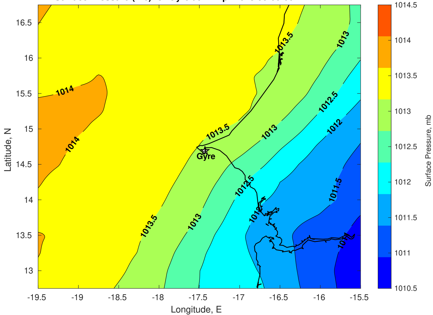
Surface Pressure (mb) for Gyre at 11-Apr-2025 00:00:00
