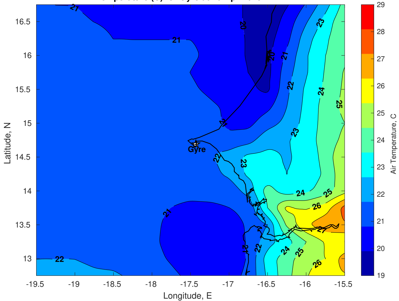
Air Temperature (C) for Gyre at 10-Apr-2025
