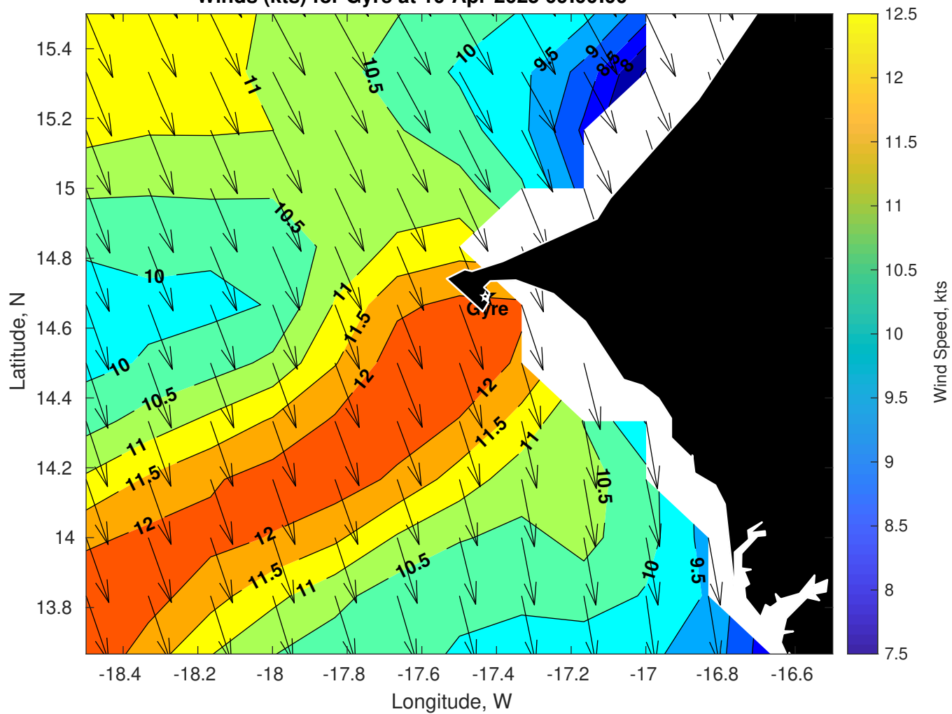
Winds (kts) for Gyre at 10-Apr-2025 09:00:00
