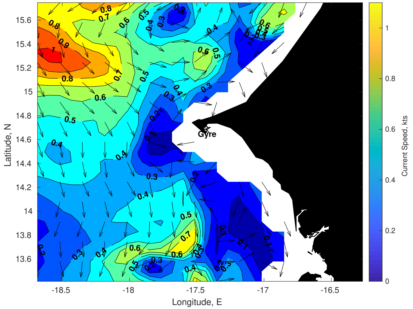
Surface Currents for Gyre at 09-Apr-2025 00:00:00
