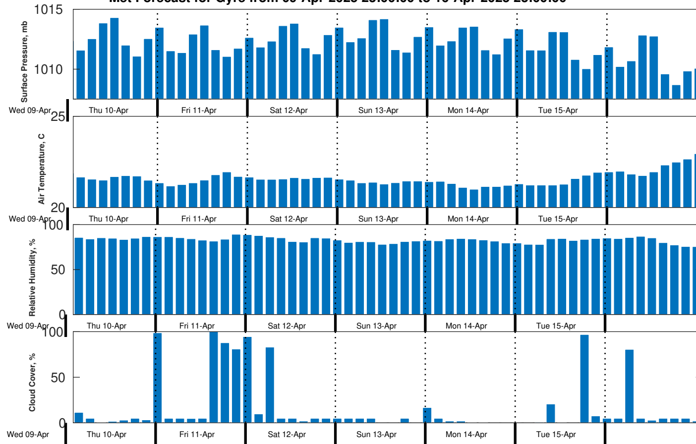
Met Forecast for Gyre from 09-Apr-2025 23:00:00 to 16-Apr-2025 23:00:00
