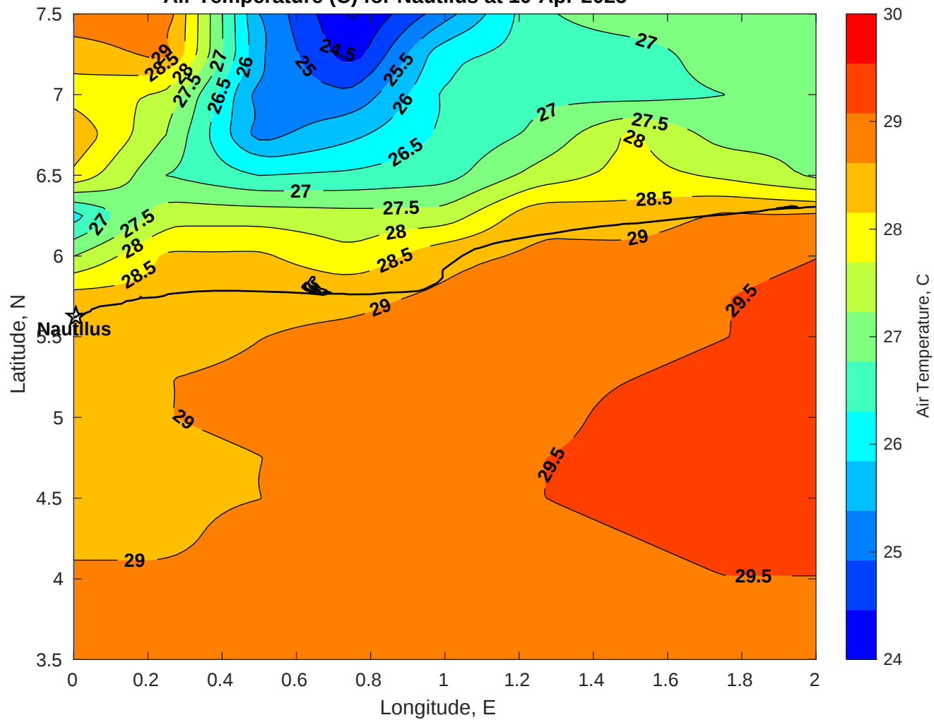
Air Temperature (C) for Nautilus at 10-Apr-2025
