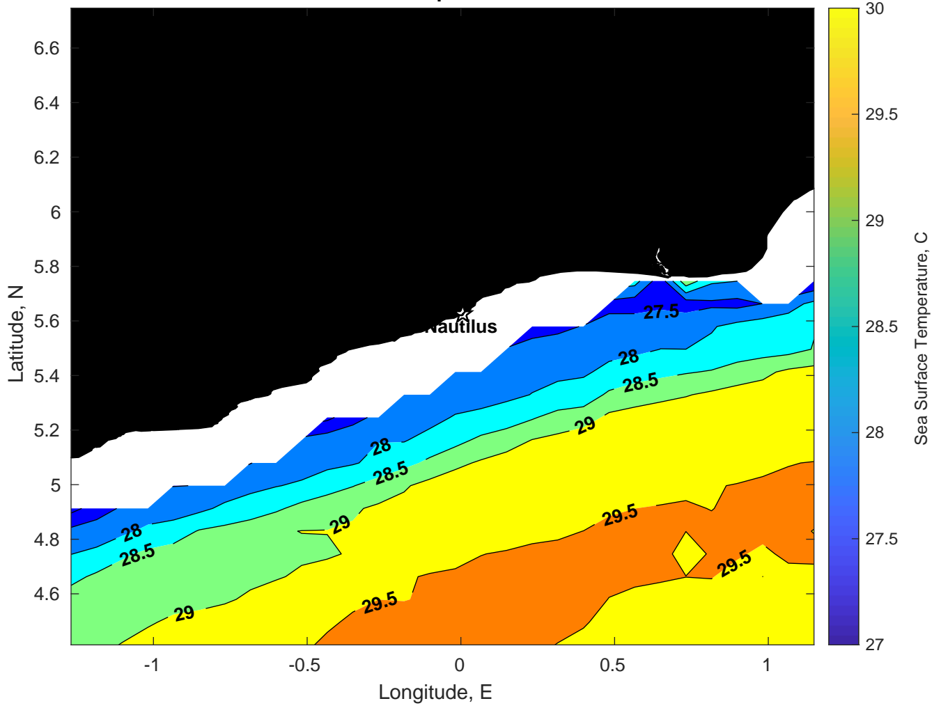
SST for Nautilus at 09-Apr-2025 00:00:00
