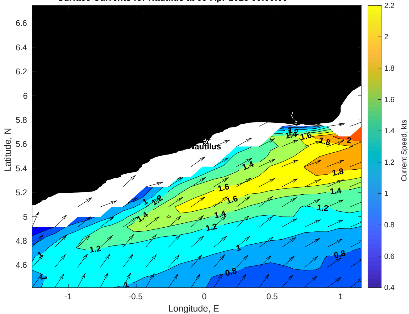
Surface Currents for Nautilus at 09-Apr-2025 00:00:00
