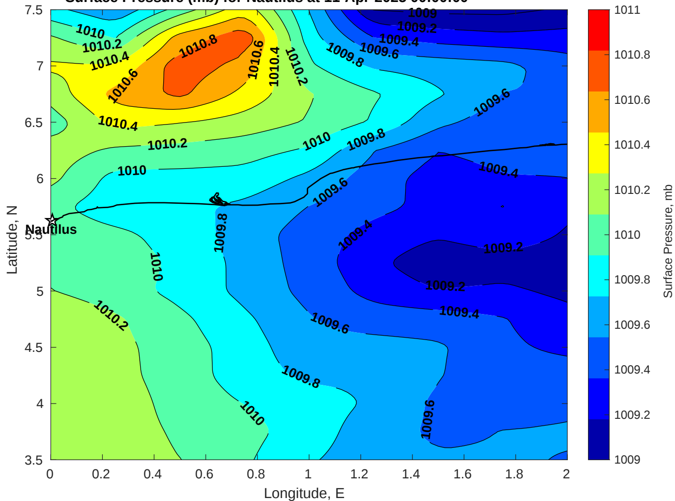
Surface Pressure (mb) for Nautilus at 11-Apr-2025 00:00:00
