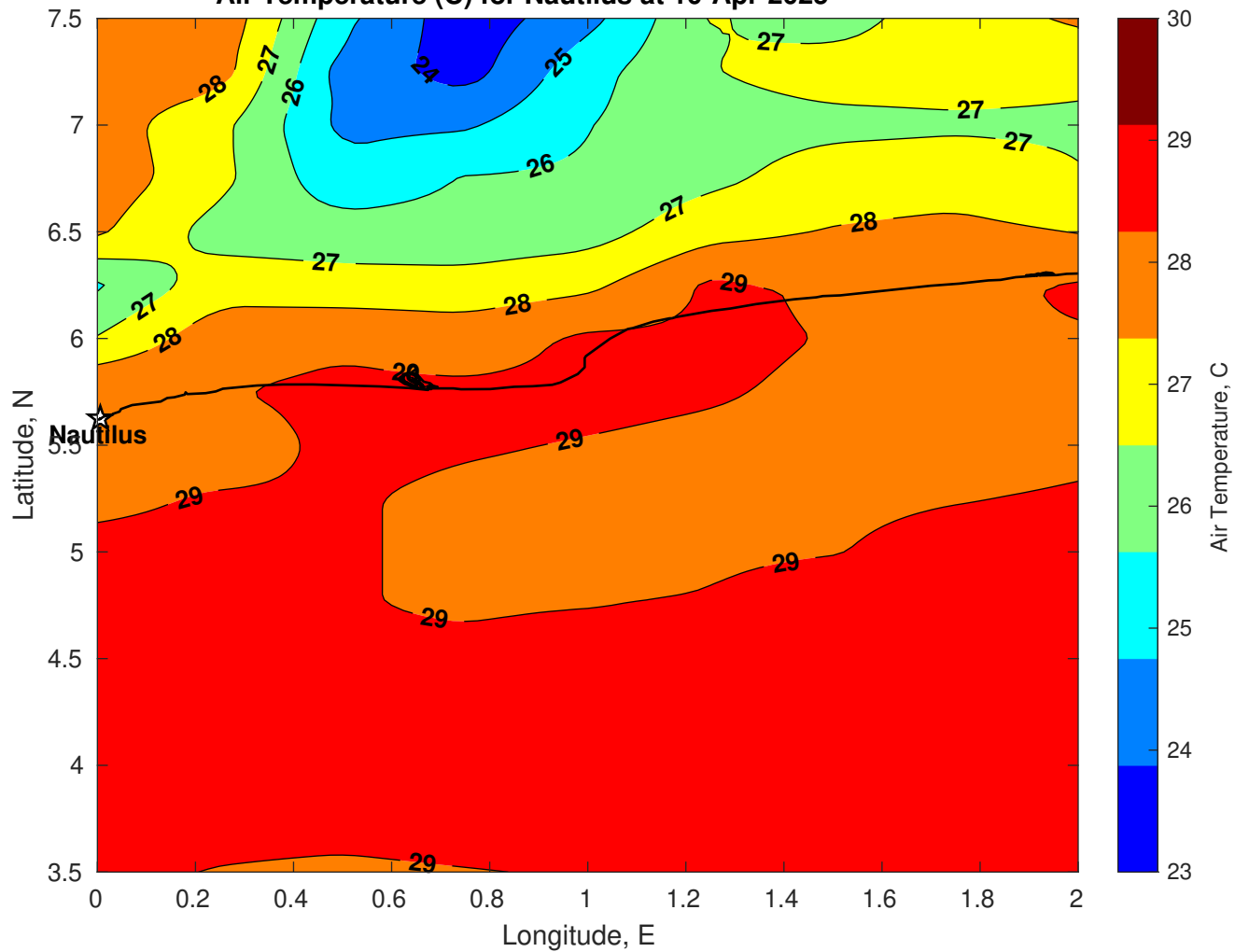
Air Temperature (C) for Nautilus at 10-Apr-2025
