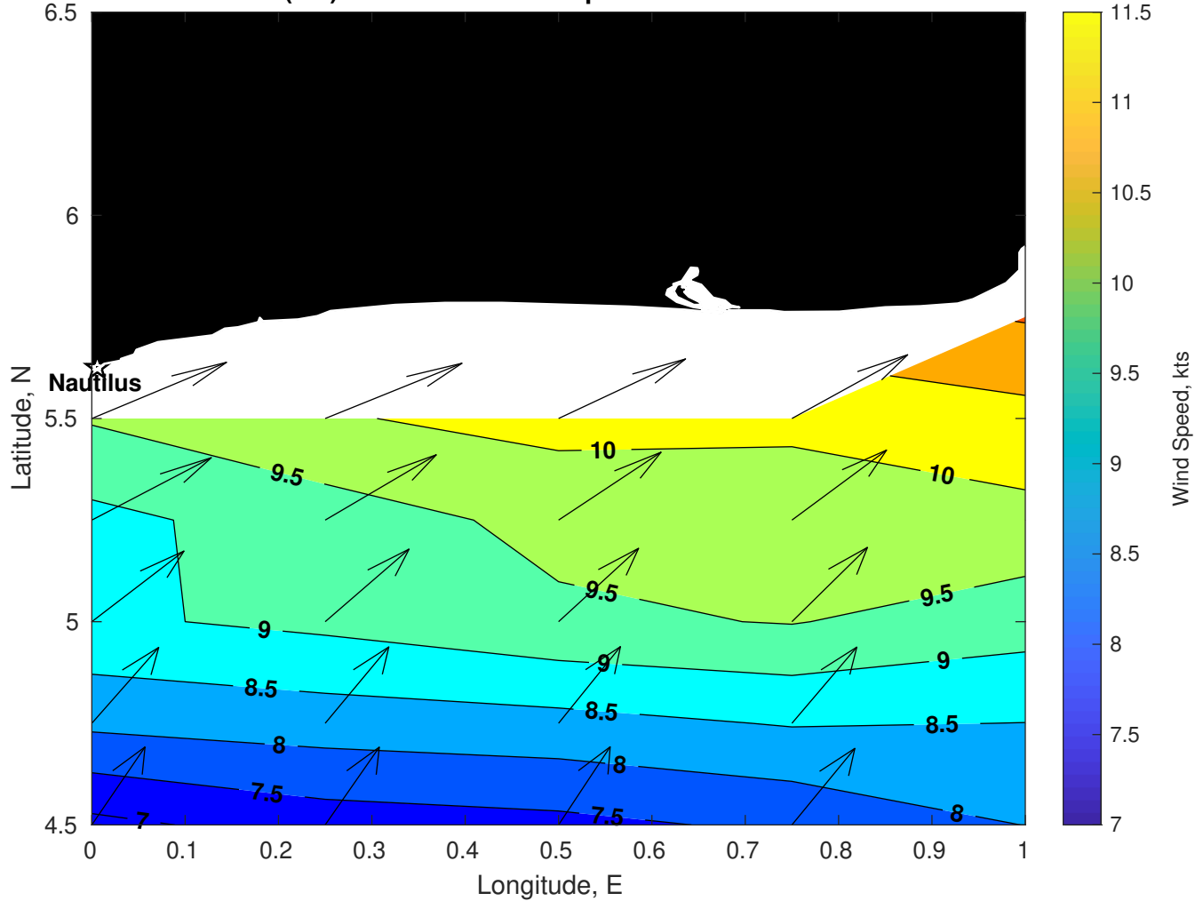
Winds (kts) for Nautilus at 10-Apr-2025 09:00:00
