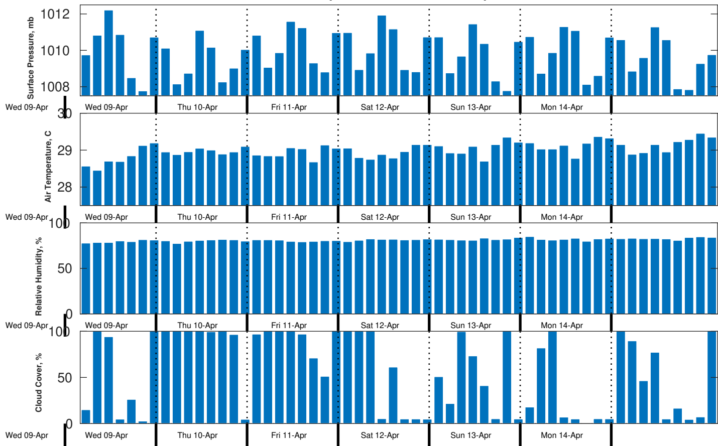
Met Forecast for Nautilus from 10-Apr-2025 00:00:00 to 17-Apr-2025 00:00:00
