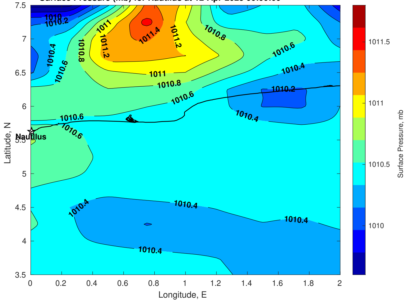
Surface Pressure (mb) for Nautilus at 12-Apr-2025 00:00:00
