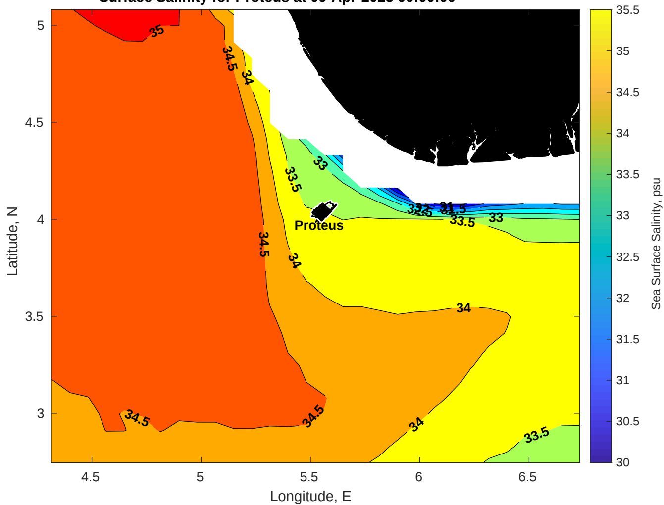
Surface Salinity for Proteus at 09-Apr-2025 00:00:00
