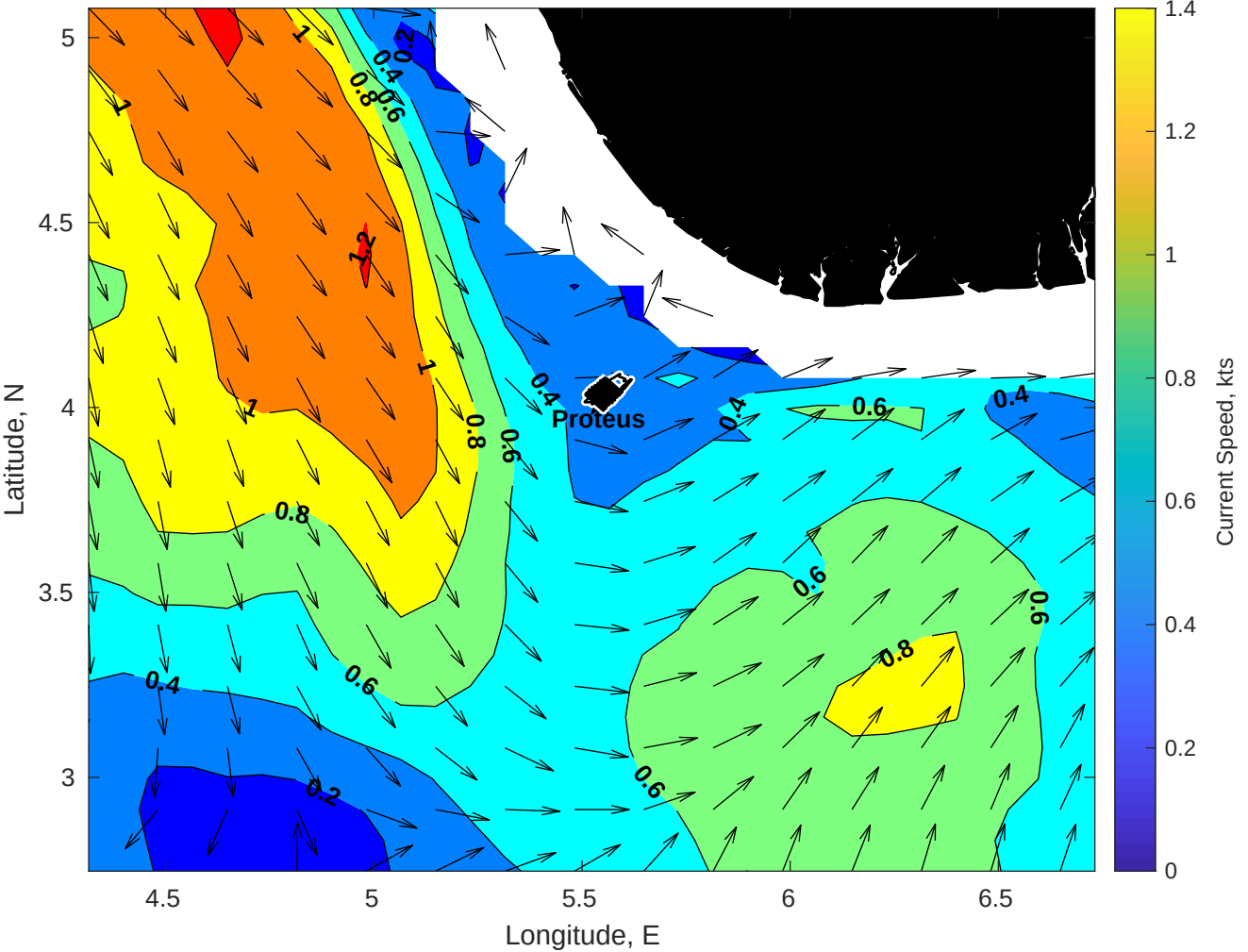
Surface Currents for Proteus at 09-Apr-2025 00:00:00
