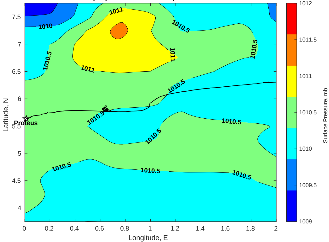
Surface Pressure (mb) for Proteus at 12-Apr-2025 00:00:00
