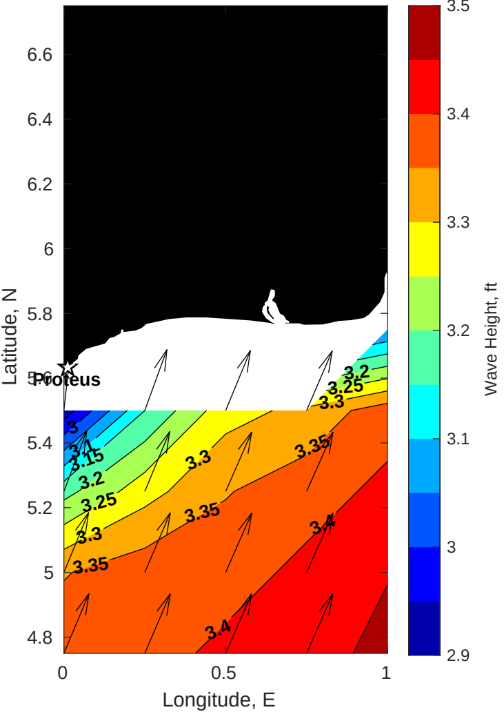
Wave Height (ft) for Proteus at 10-Apr-2025 09:00:00
