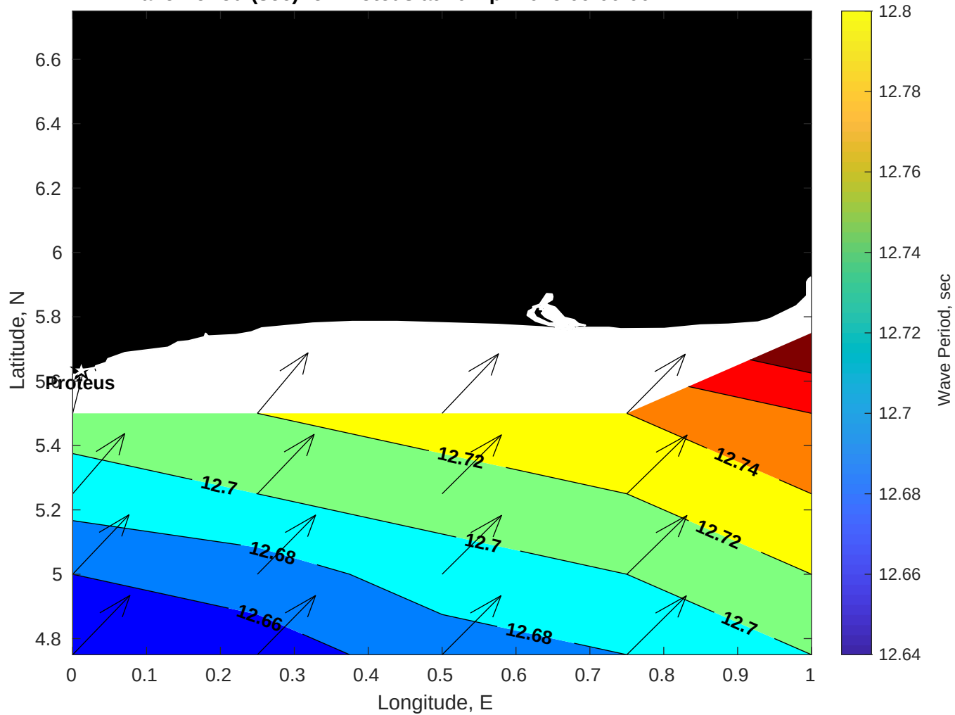
Wave Period (sec) for Proteus at 10-Apr-2025 09:00:00
