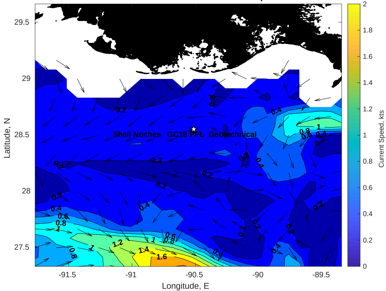
Surface Currents for Shell Noches GC19 PPL Geotechnical at 09-Apr-2025 00:00:00
