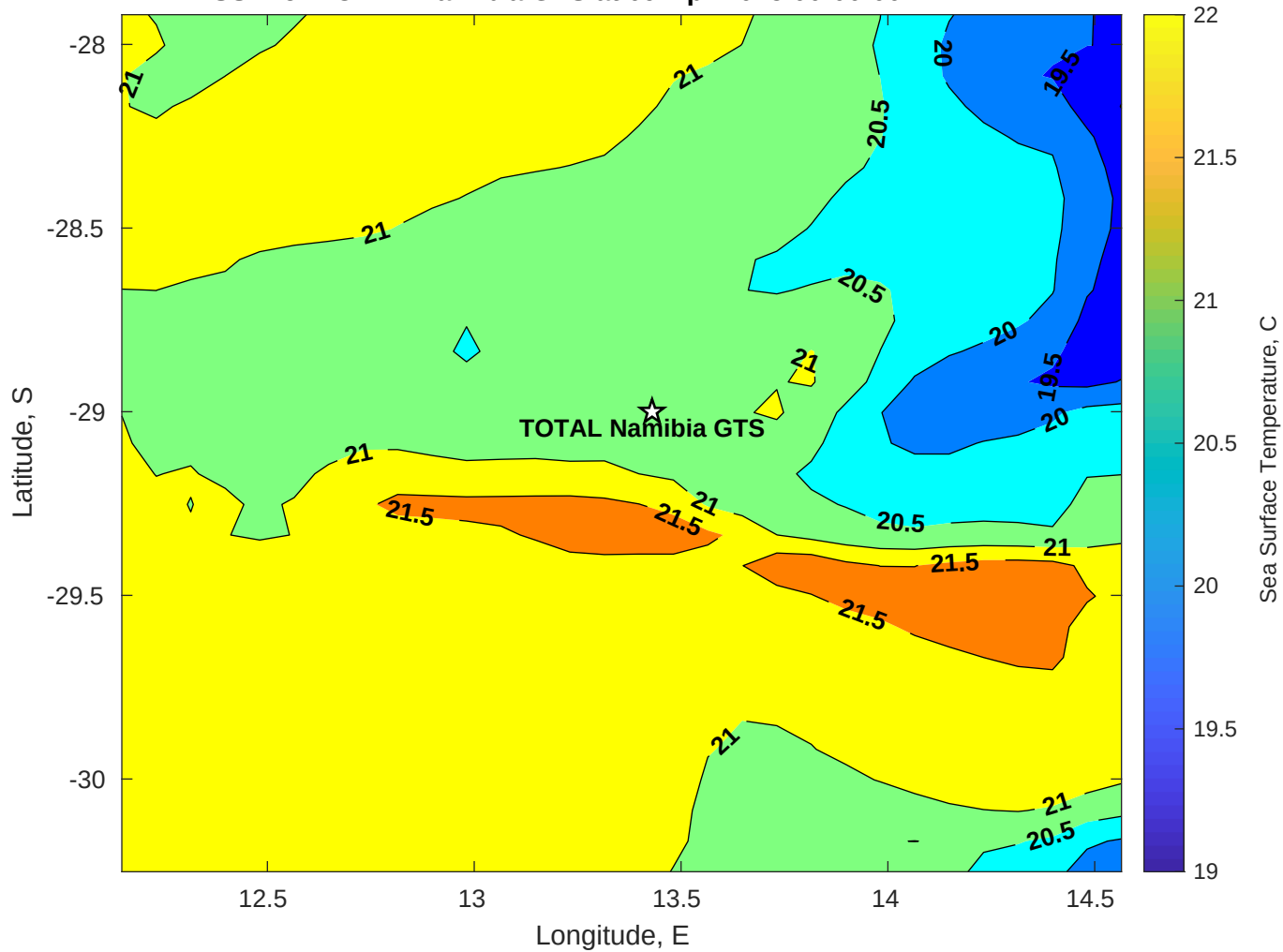
SST for TOTAL Namibia GTS at 09-Apr-2025 00:00:00
