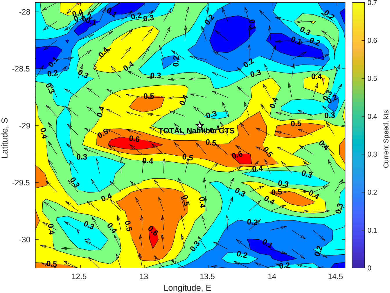
Surface Currents for TOTAL Namibia GTS at 09-Apr-2025 00:00:00
