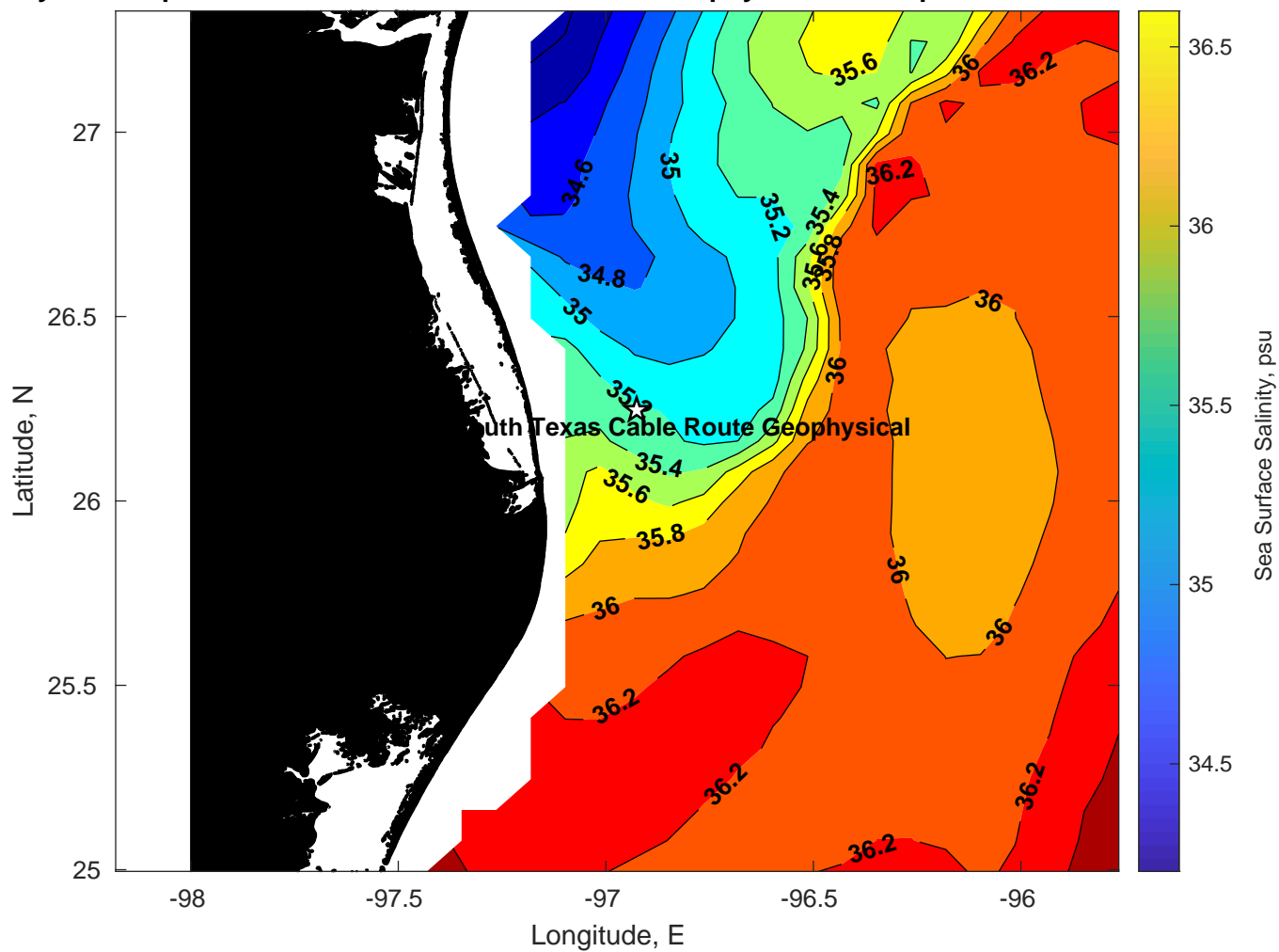
Surface Salinity for Tampnet P2378 South Texas Cable Route Geophysical at 09-Apr-2025 00:00:00
