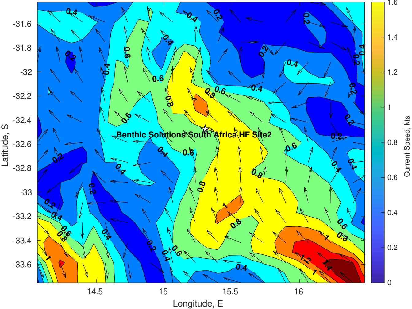
Surface Currents for Benthic Solutions South Africa HF Site2 at 10-Apr-2025 00:00:00
