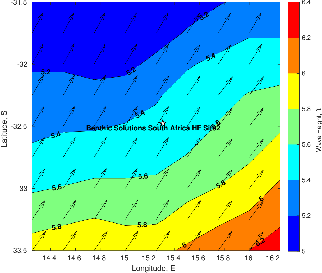
Wave Height (ft) for Benthic Solutions South Africa HF Site2 at 11-Apr-2025 09:00:00
