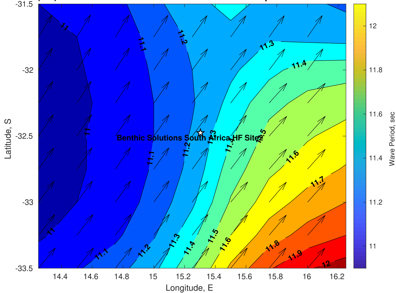
Wave Period (sec) for Benthic Solutions South Africa HF Site2 at 11-Apr-2025 09:00:00
