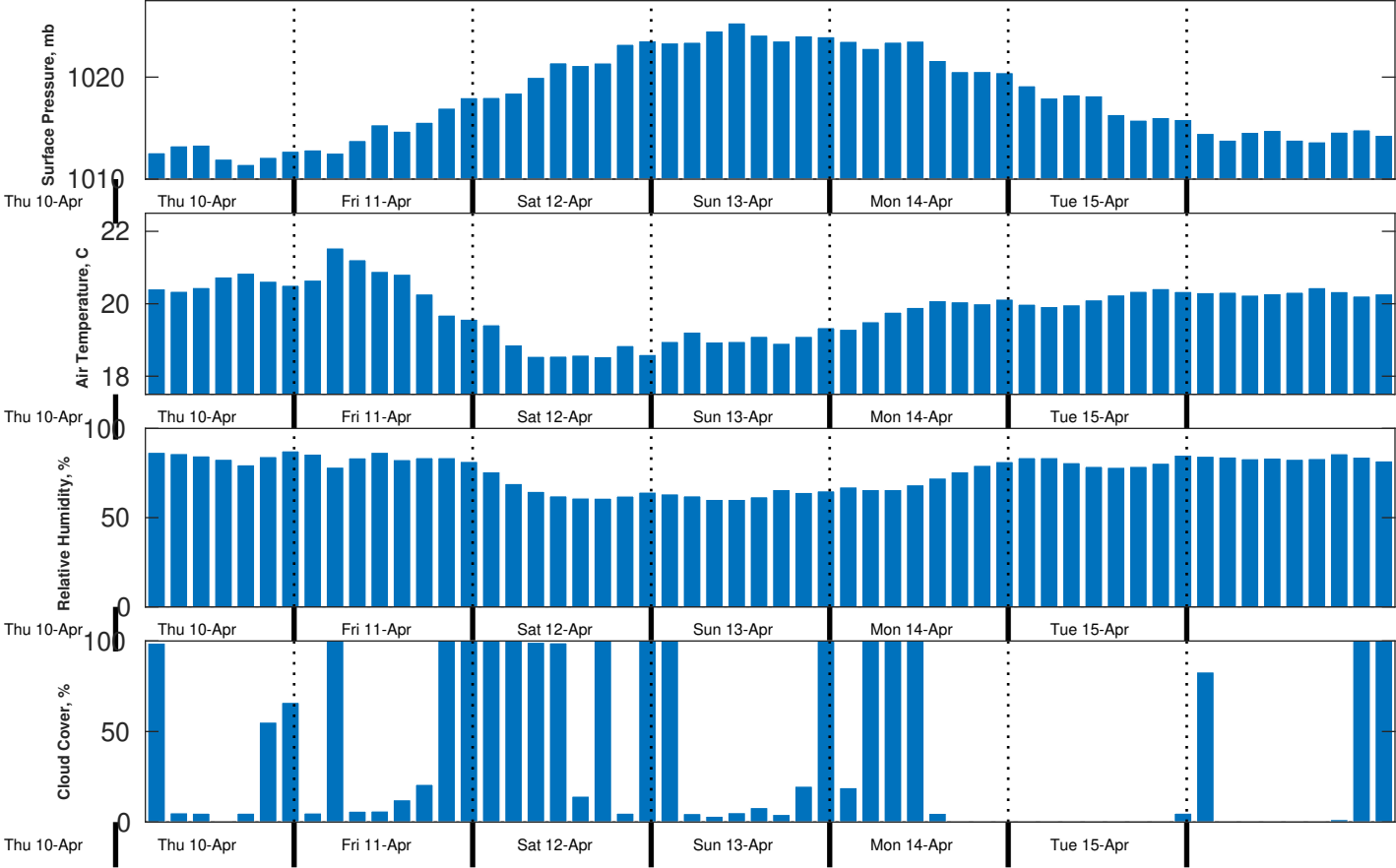
Met Forecast for Benthic Solutions South Africa HF Site2 from 11-Apr-2025 00:00:00 to 18-Apr-2025 00:00:00
