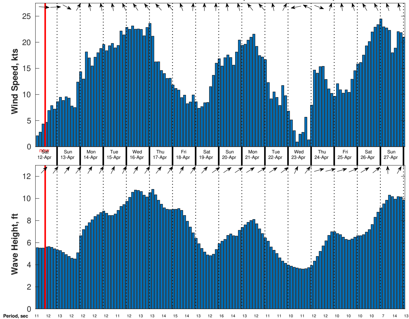
Wind & Wave Forecast for Benthic Solutions South Africa HF Site3 from 11-Apr-2025 02:00:00 to 27-Apr-2025 02:00:00
