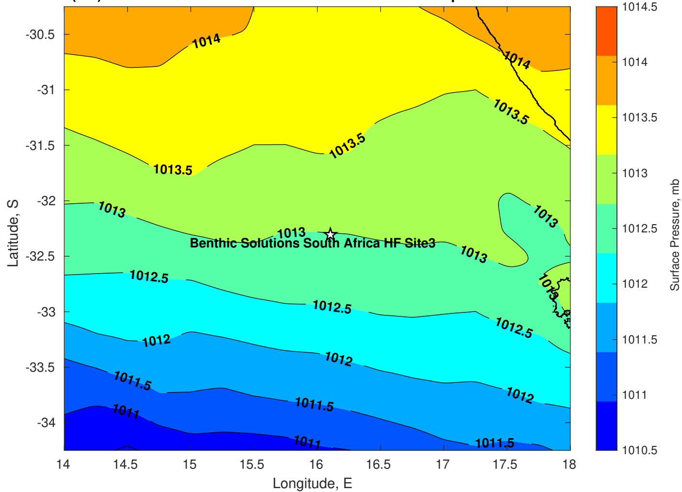
Surface Pressure (mb) for Benthic Solutions South Africa HF Site3 at 12-Apr-2025 00:00:00
