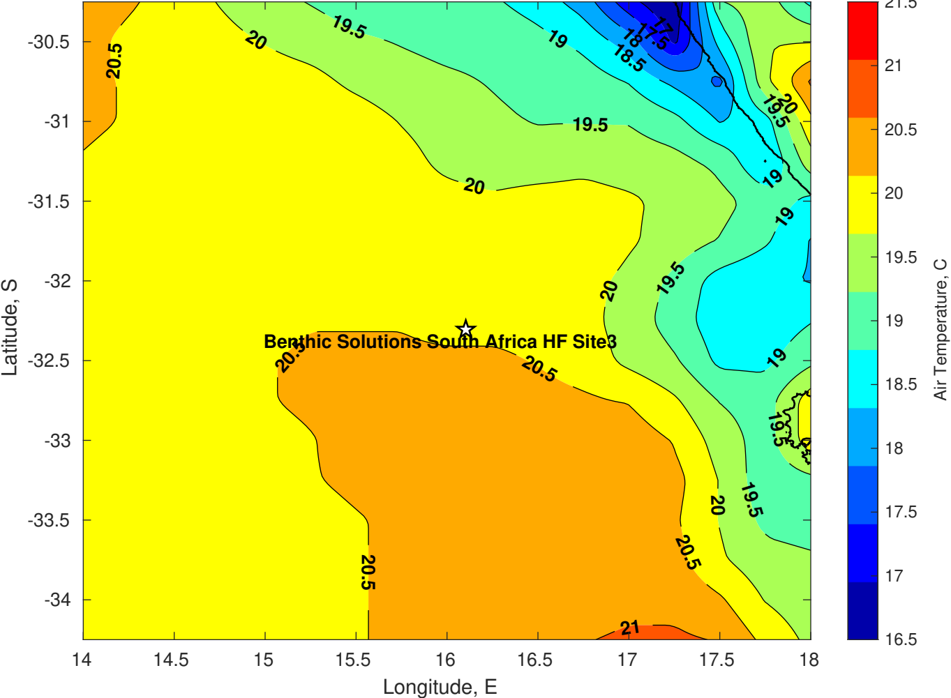
Air Temperature (C) for Benthic Solutions South Africa HF Site3 at 11-Apr-2025
