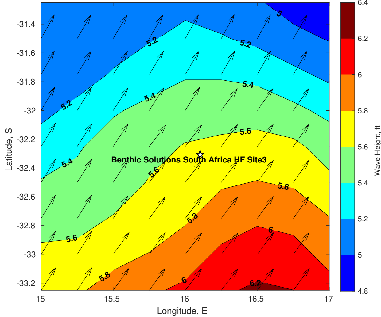
Wave Height (ft) for Benthic Solutions South Africa HF Site3 at 11-Apr-2025 09:00:00
