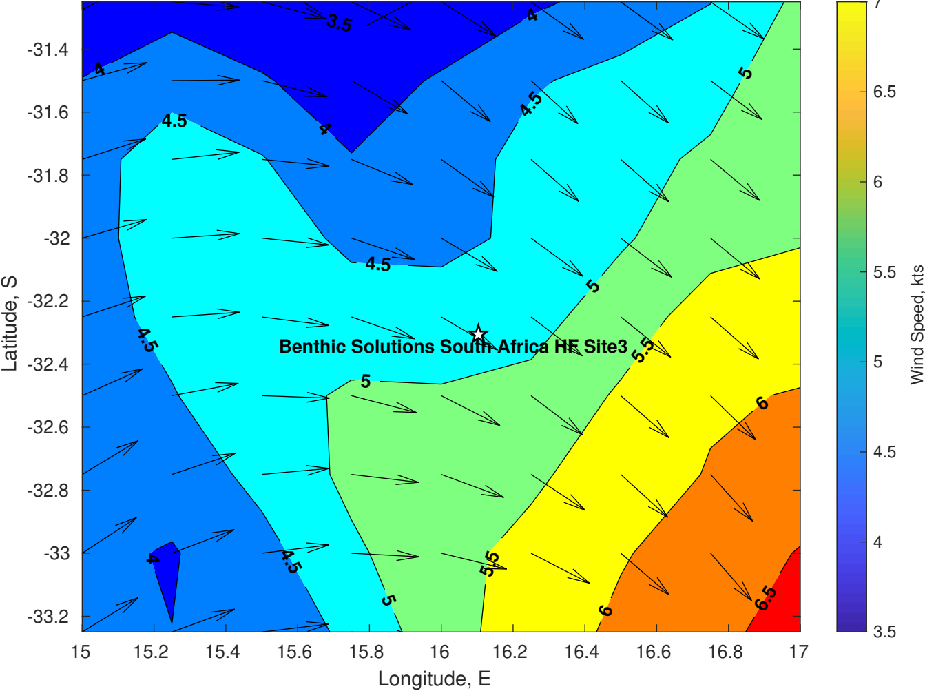
Winds (kts) for Benthic Solutions South Africa HF Site3 at 11-Apr-2025 09:00:00
