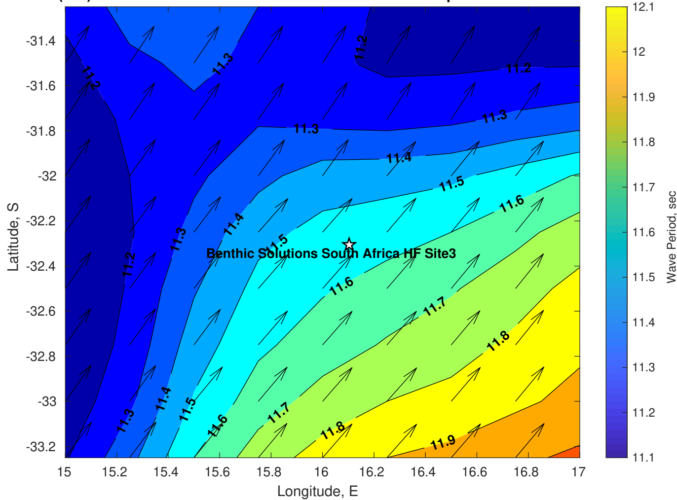
Wave Period (sec) for Benthic Solutions South Africa HF Site3 at 11-Apr-2025 09:00:00
