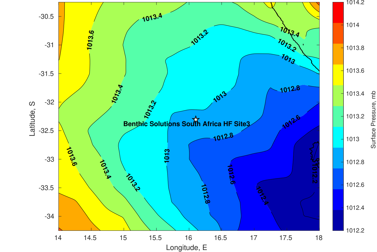
Surface Pressure (mb) for Benthic Solutions South Africa HF Site3 at 11-Apr-2025 00:00:00
