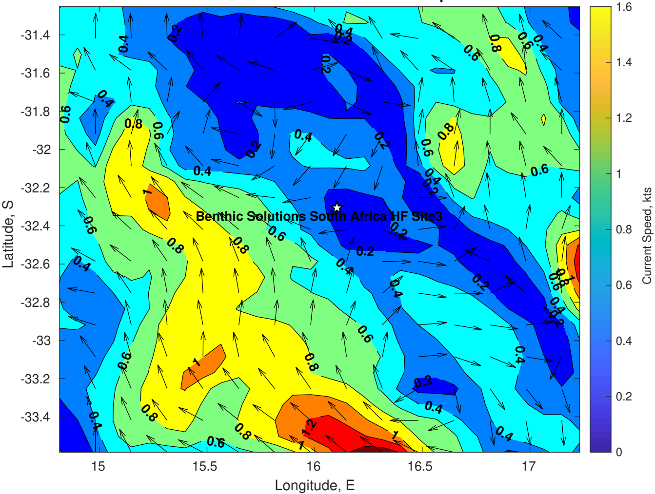
Surface Currents for Benthic Solutions South Africa HF Site3 at 10-Apr-2025 00:00:00
