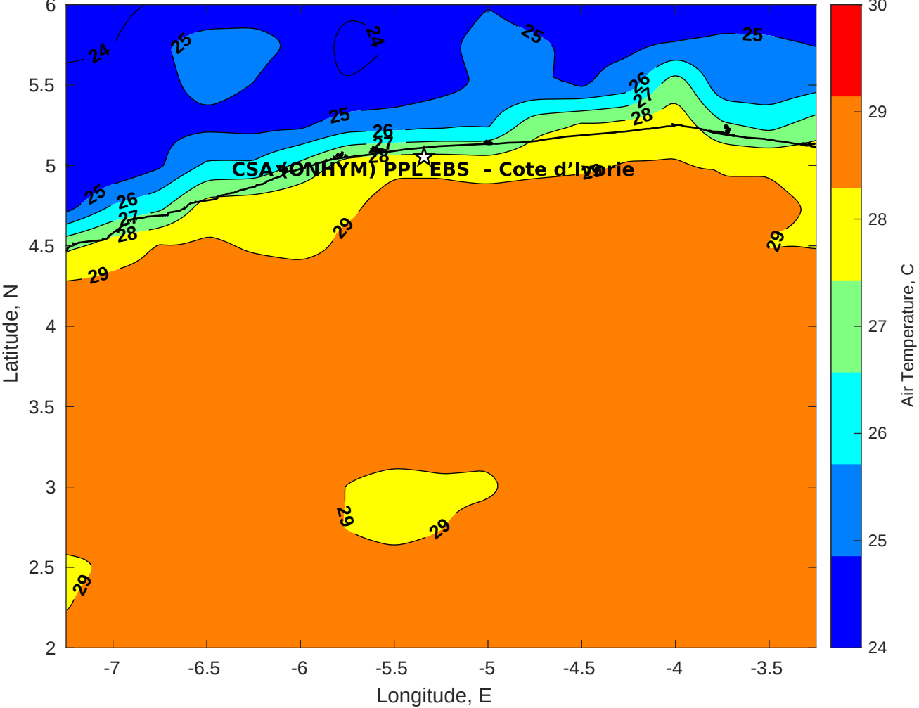
Air Temperature (C) for CSA (ONHYM) PPL EBS - Cote d'Ivoire at 11-Apr-2025
