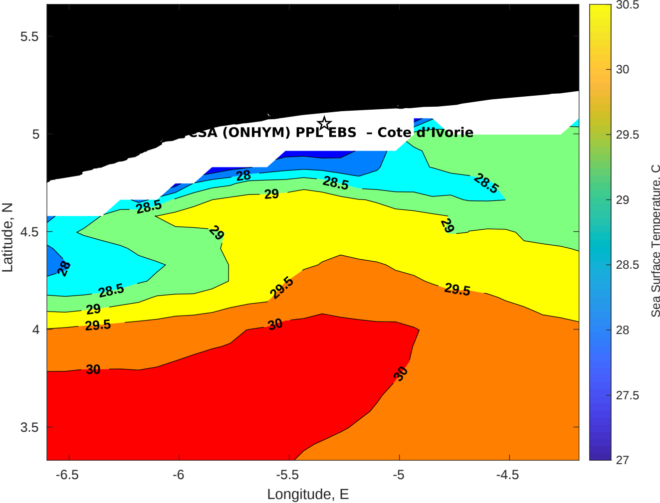
SST for CSA (ONHYM) PPL EBS - Cote d'Ivoire at 10-Apr-2025 00:00:00
