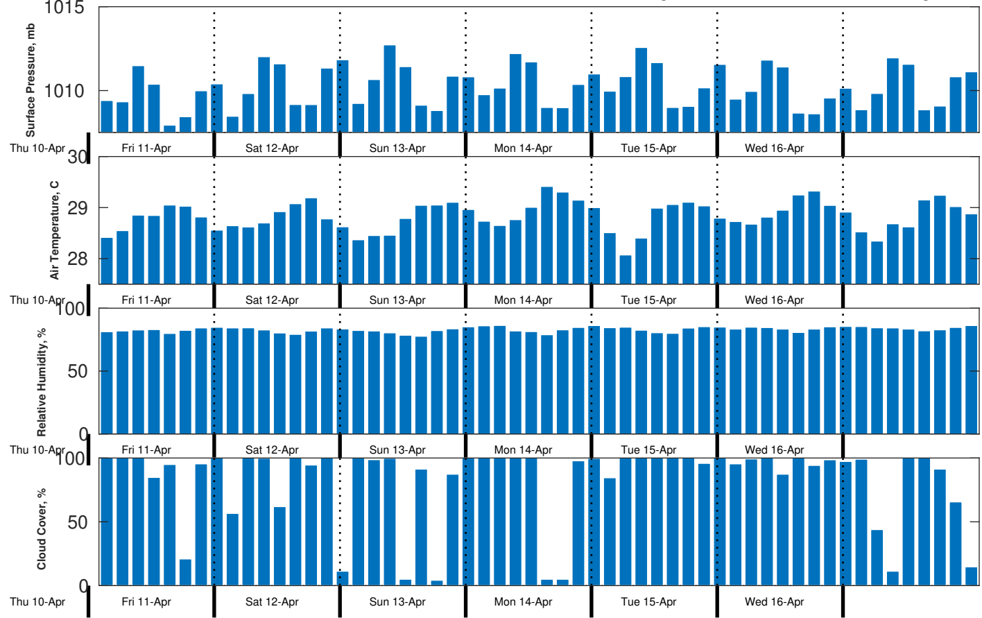
Met Forecast for CSA (ONHYM) PPL EBS - Cote d'Ivoire from 11-Apr-2025 00:00:00 to 18-Apr-2025 00:00:00
