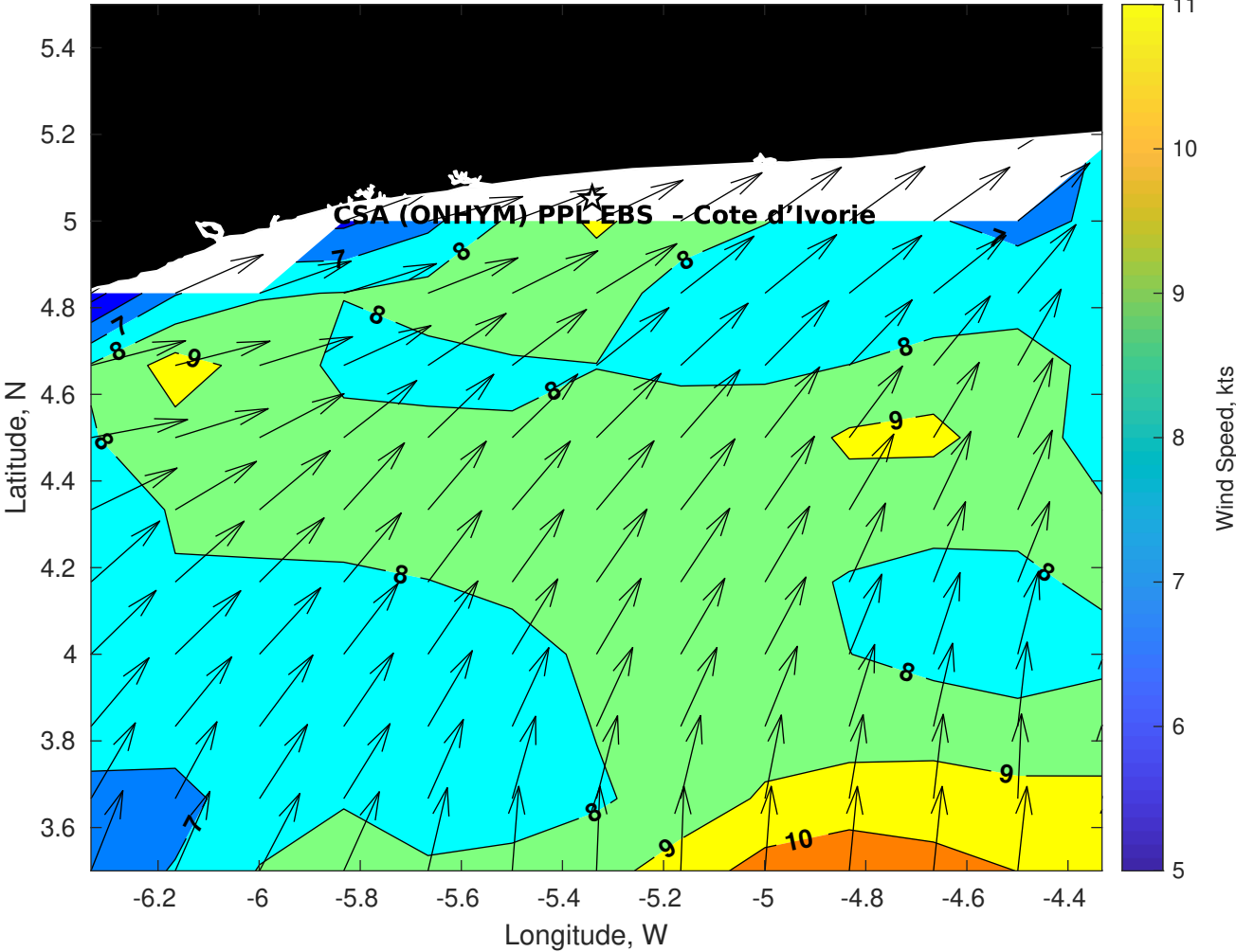
Winds (kts) for CSA (ONHYM) PPL EBS - Cote d'Ivoire at 11-Apr-2025 09:00:00
