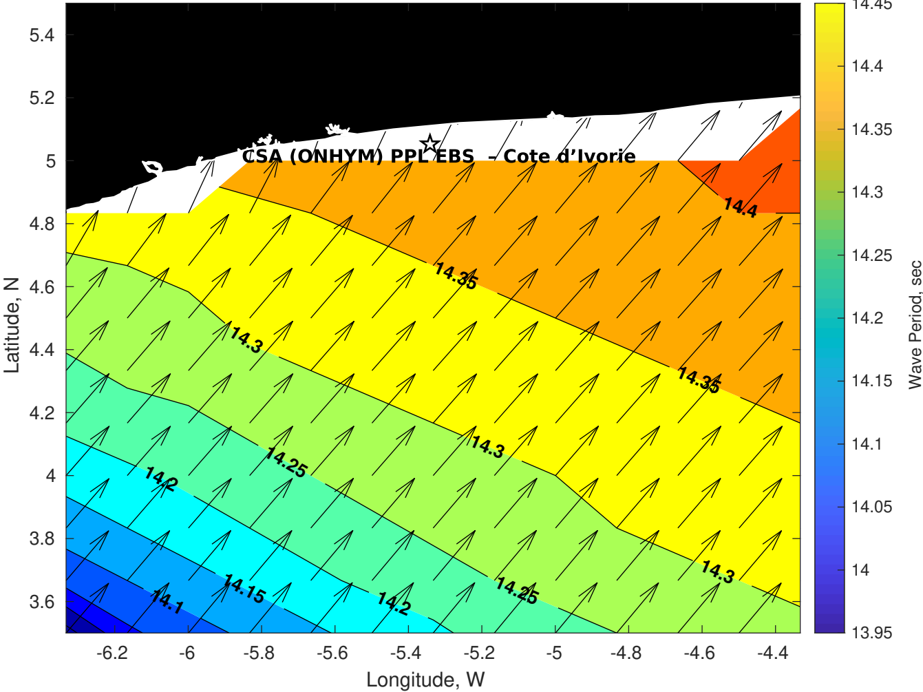
Wave Period (sec) for CSA (ONHYM) PPL EBS - Cote d'Ivoire at 11-Apr-2025 09:00:00
