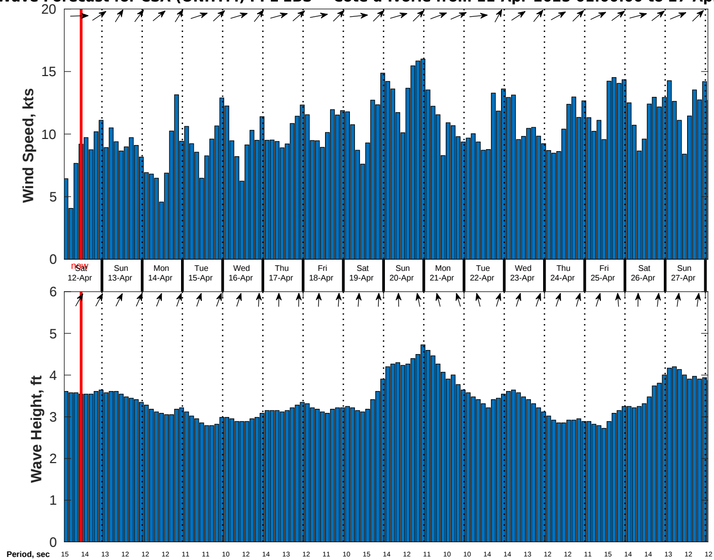
Wind & Wave Forecast for CSA (ONHYM) PPL EBS - Cote d'Ivoire from 11-Apr-2025 01:00:00 to 27-Apr-2025 01:00:00
