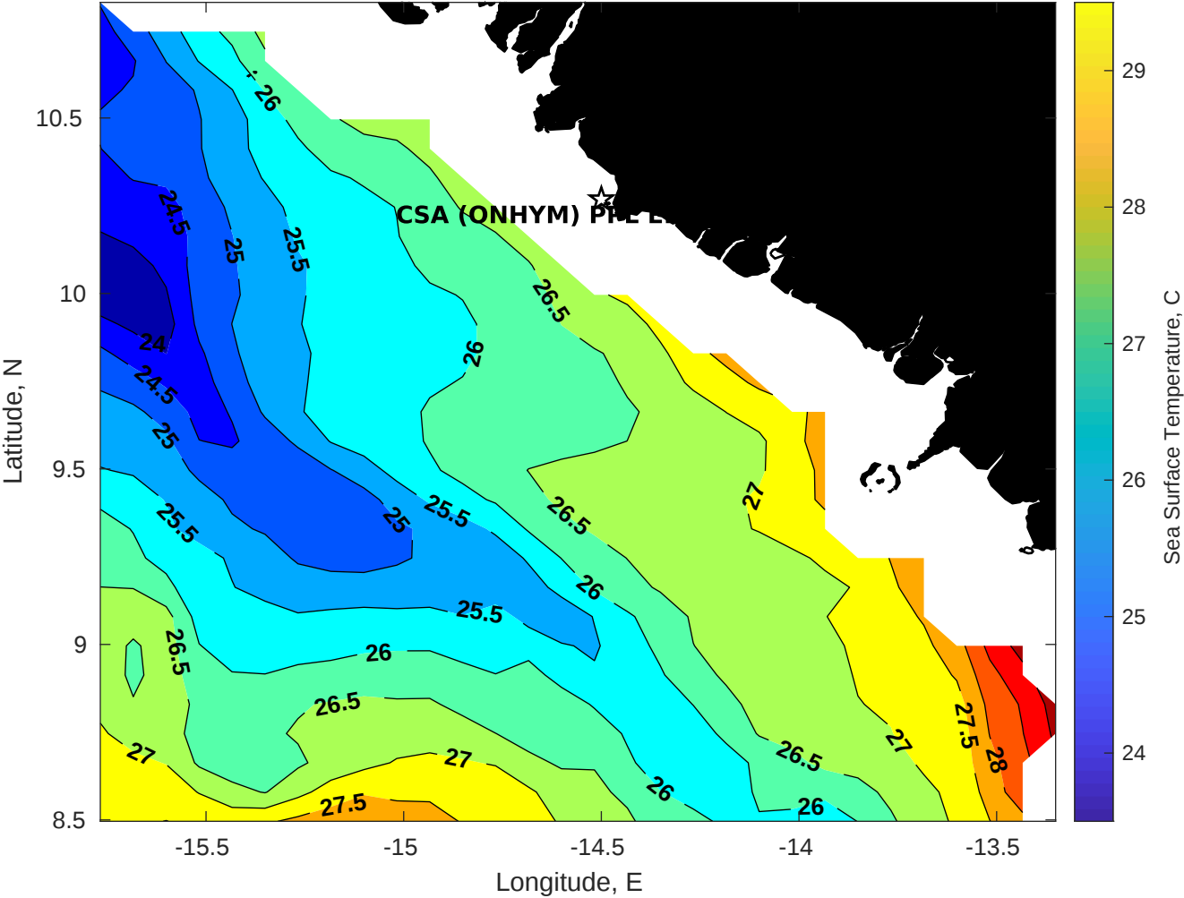
SST for CSA (ONHYM) PPL EBS - Guinea at 10-Apr-2025 00:00:00
