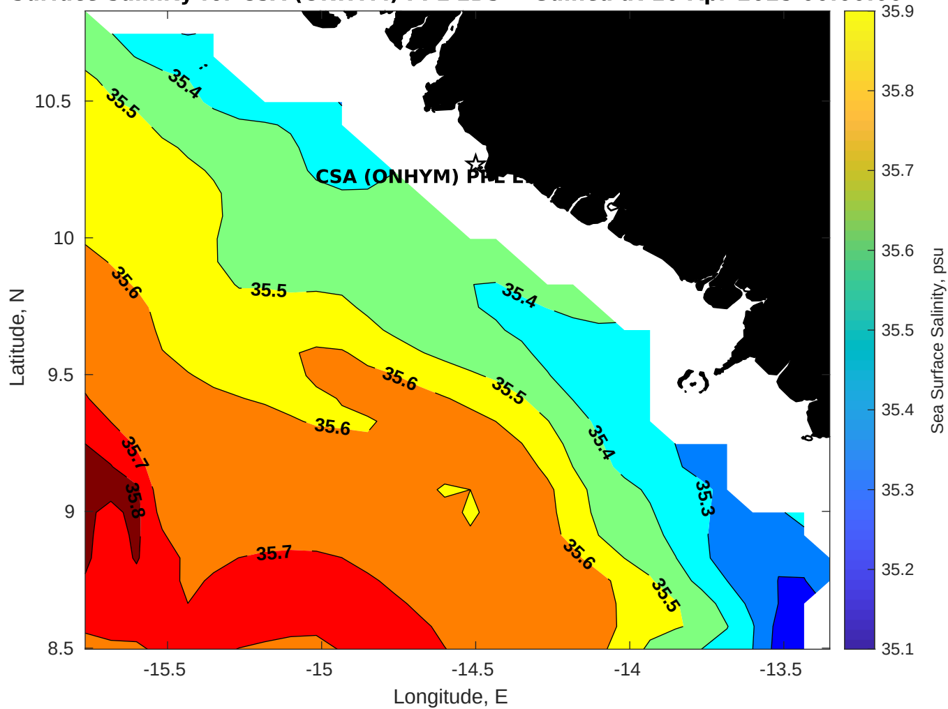
Surface Salinity for CSA (ONHYM) PPL EBS - Guinea at 10-Apr-2025 00:00:00
