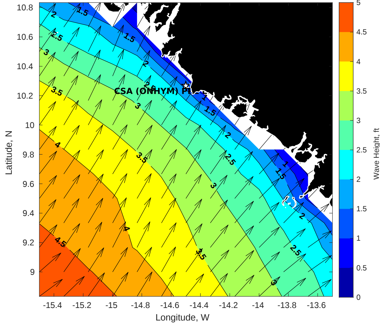
Wave Height (ft) for CSA (ONHYM) PPL EBS - Guinea at 11-Apr-2025 09:00:00
