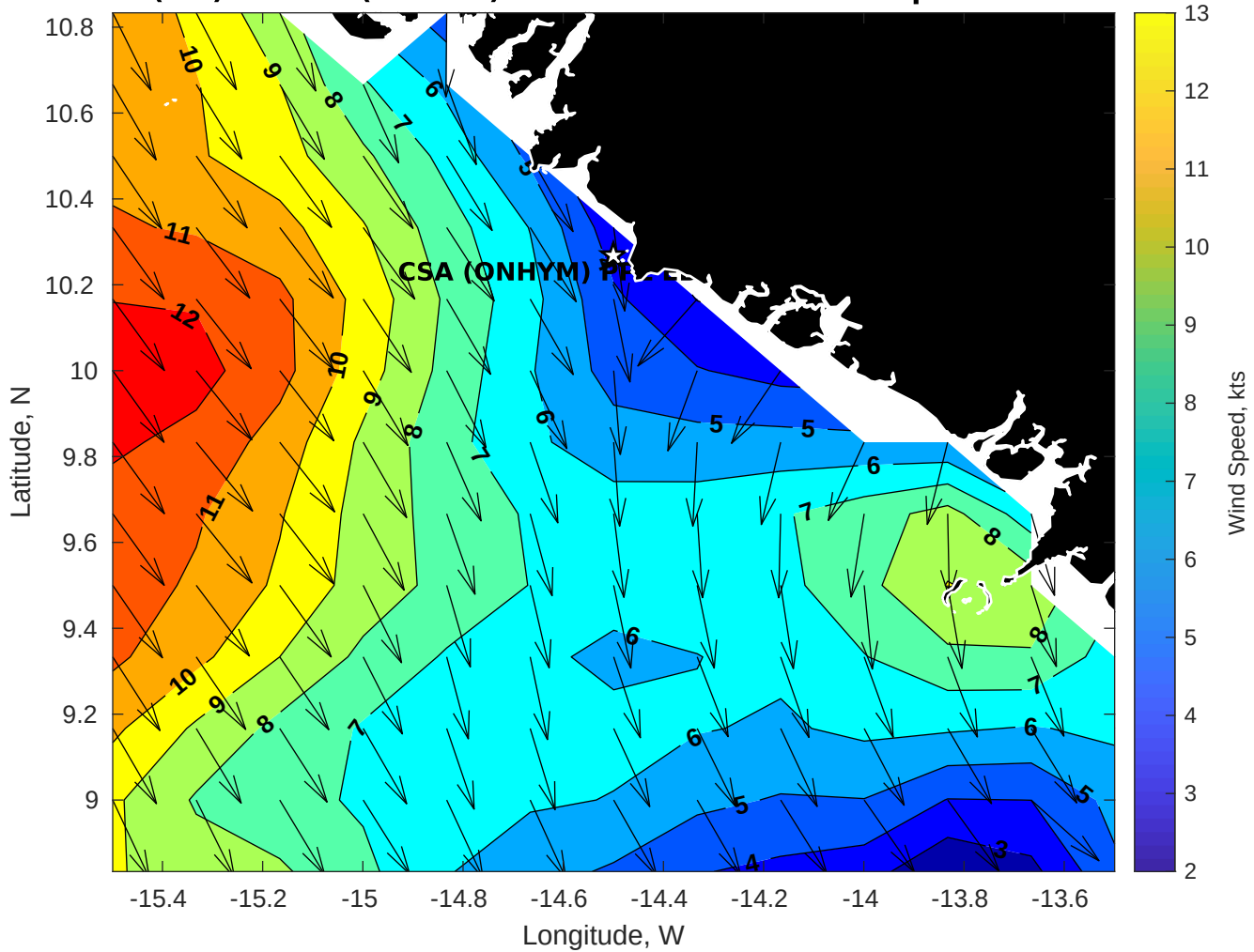
Winds (kts) for CSA (ONHYM) PPL EBS - Guinea at 11-Apr-2025 09:00:00
