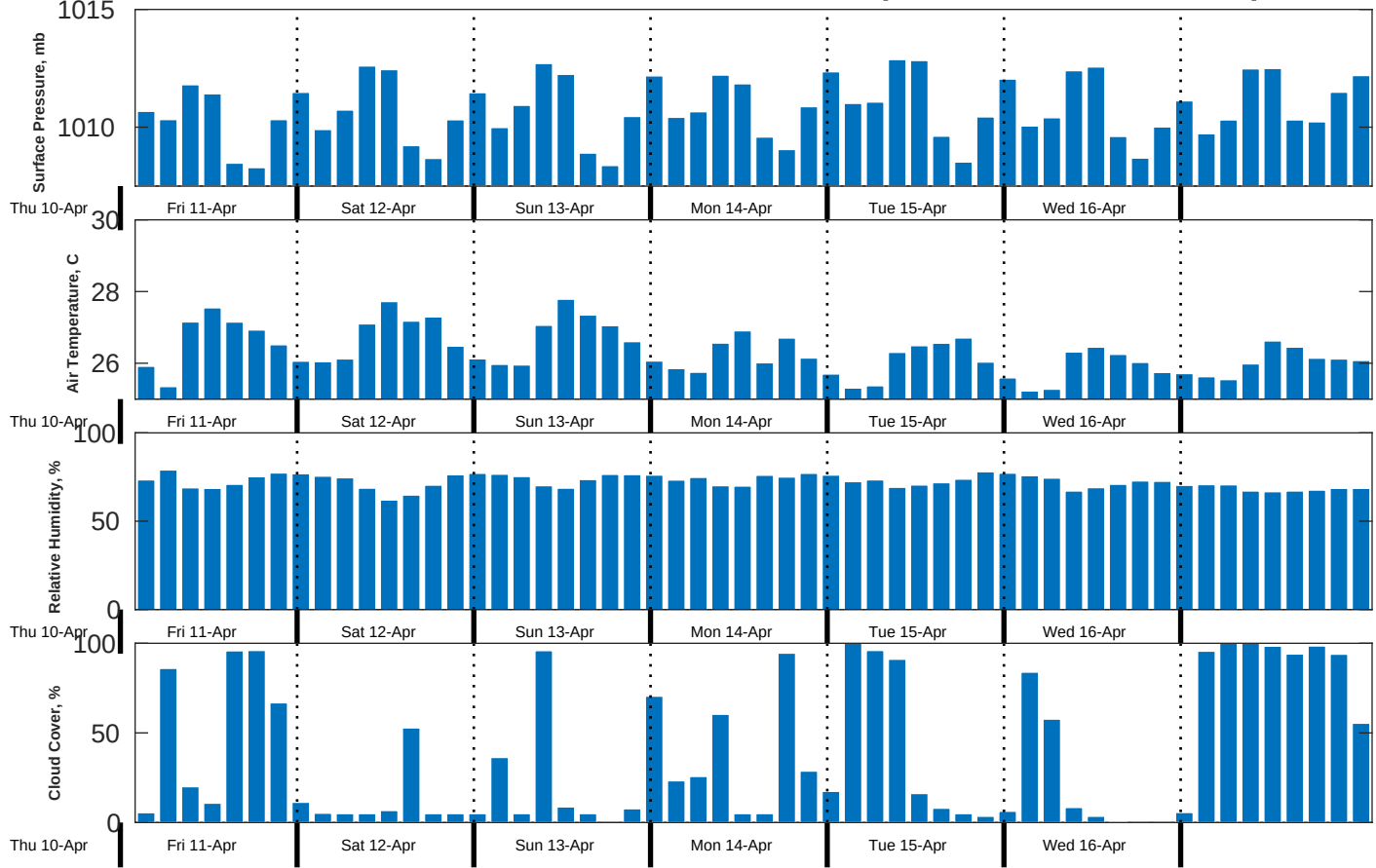
Met Forecast for CSA (ONHYM) PPL EBS - Guinea from 11-Apr-2025 00:00:00 to 18-Apr-2025 00:00:00
