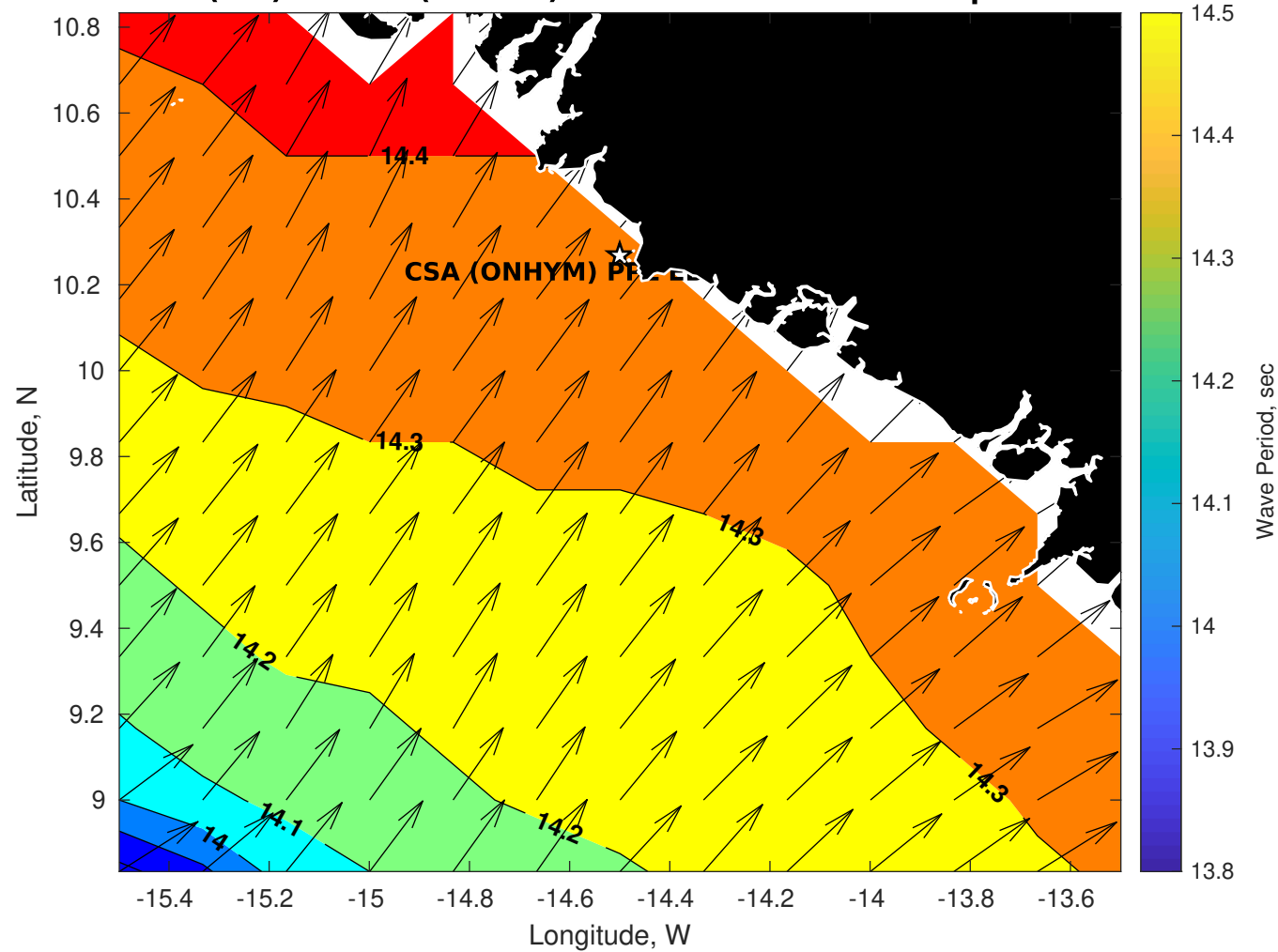
Wave Period (sec) for CSA (ONHYM) PPL EBS - Guinea at 11-Apr-2025 09:00:00
