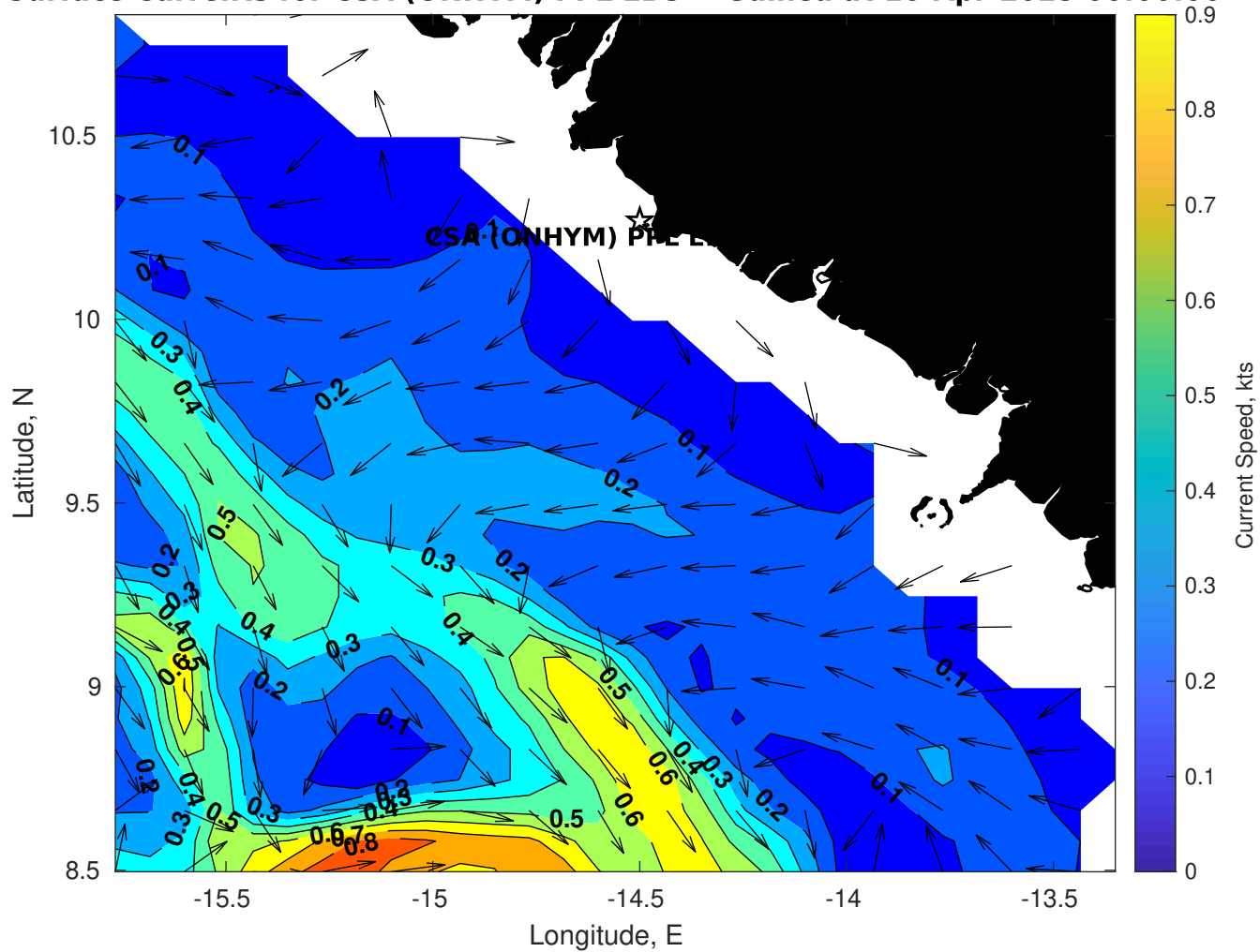
Surface Currents for CSA (ONHYM) PPL EBS - Guinea at 10-Apr-2025 00:00:00
