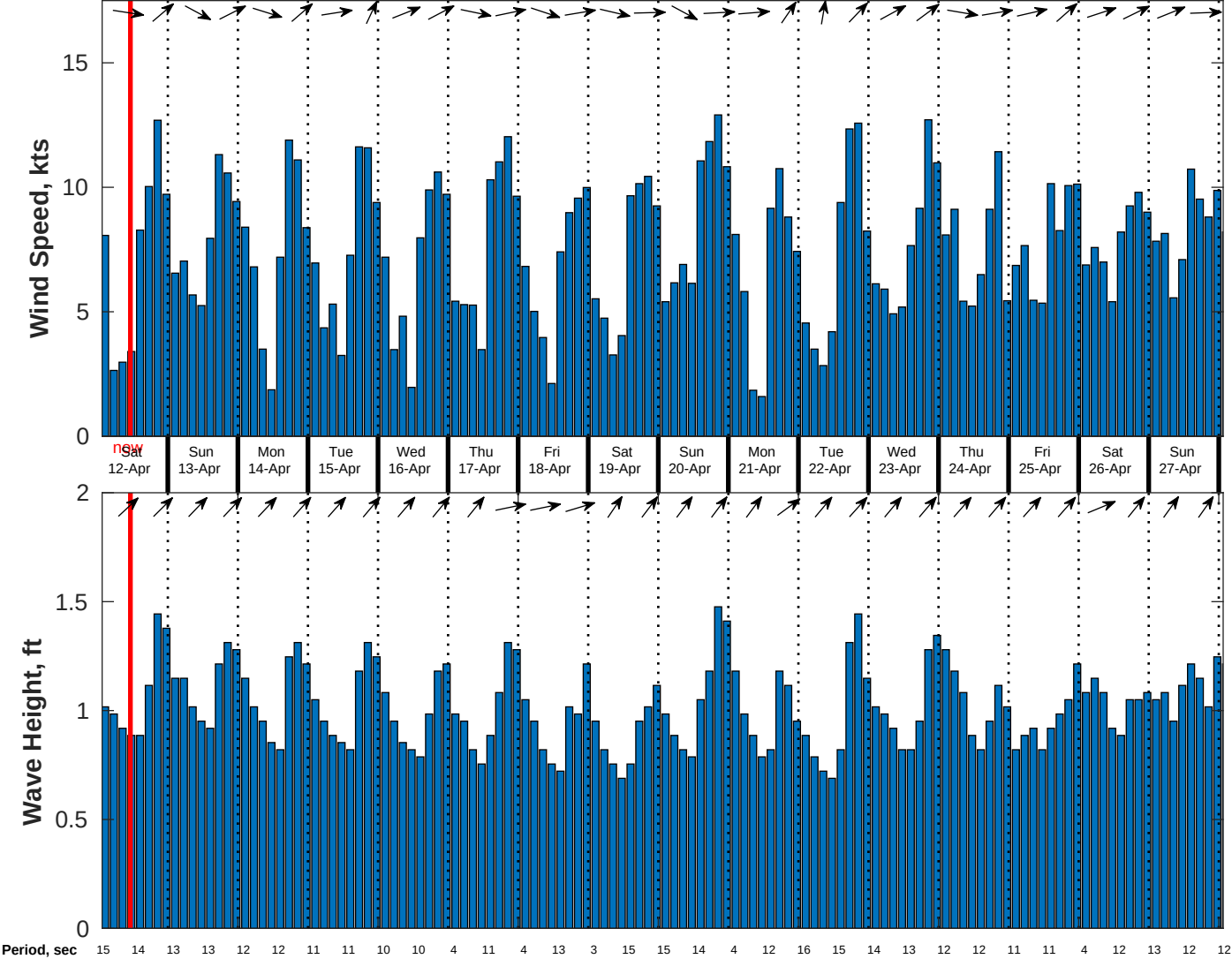
Wind & Wave Forecast for CSA (ONHYM) PPL EBS - Guinea from 11-Apr-2025 01:00:00 to 27-Apr-2025 01:00:00
