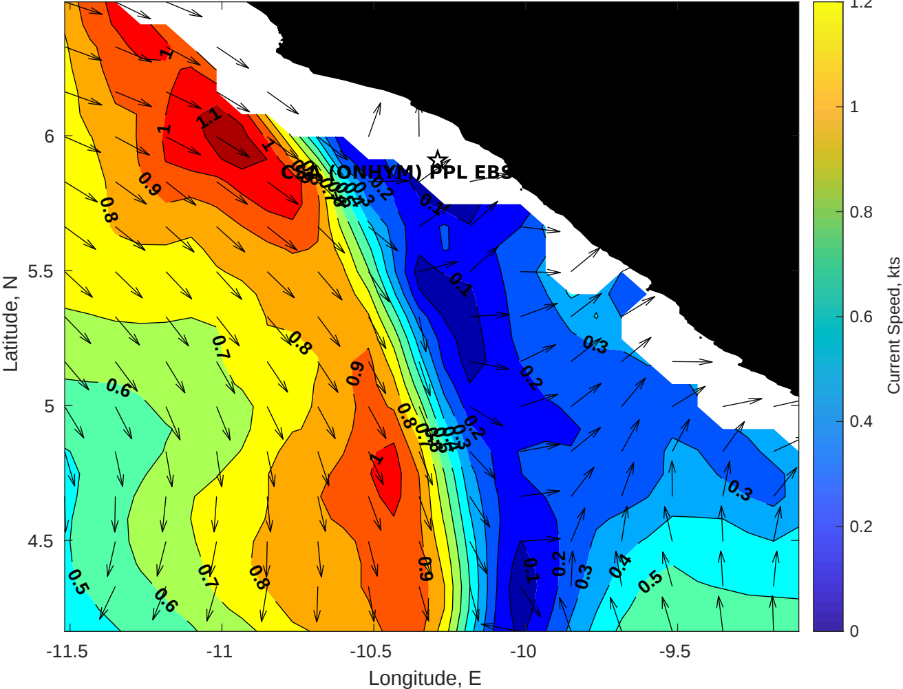
Surface Currents for CSA (ONHYM) PPL EBS - Liberia at 10-Apr-2025 00:00:00
