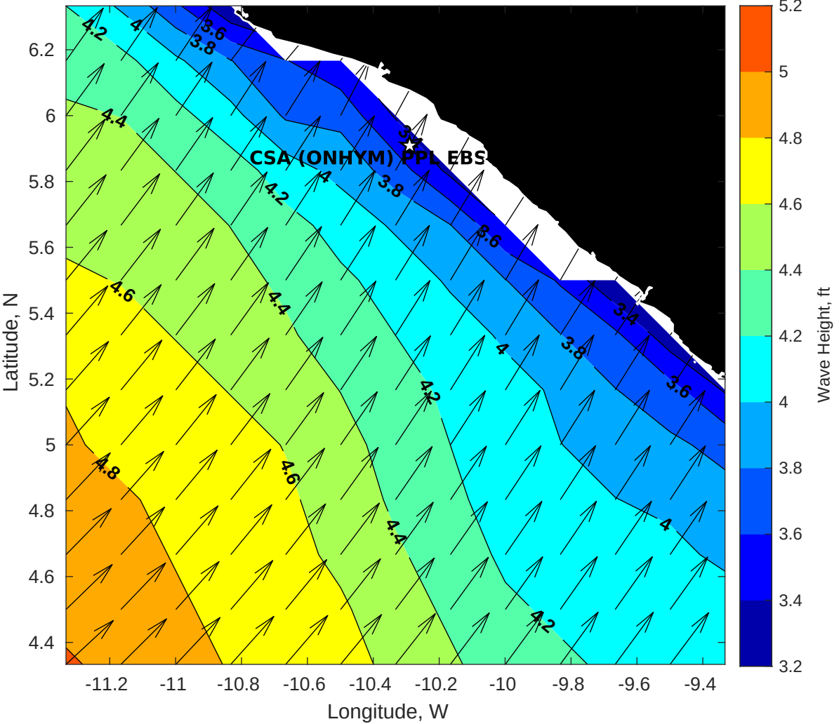
Wave Height (ft) for CSA (ONHYM) PPL EBS - Liberia at 11-Apr-2025 09:00:00
