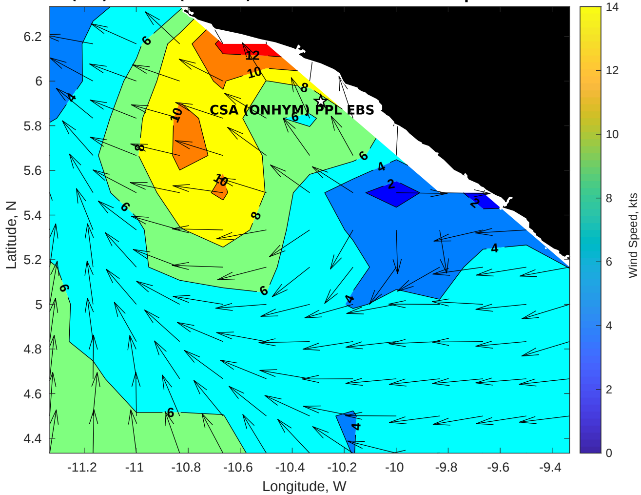
Winds (kts) for CSA (ONHYM) PPL EBS - Liberia at 11-Apr-2025 09:00:00
