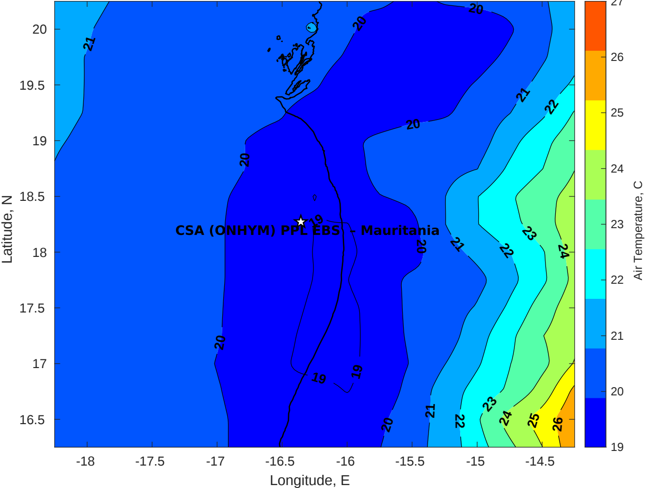
Air Temperature (C) for CSA (ONHYM) PPL EBS - Mauritania at 11-Apr-2025
