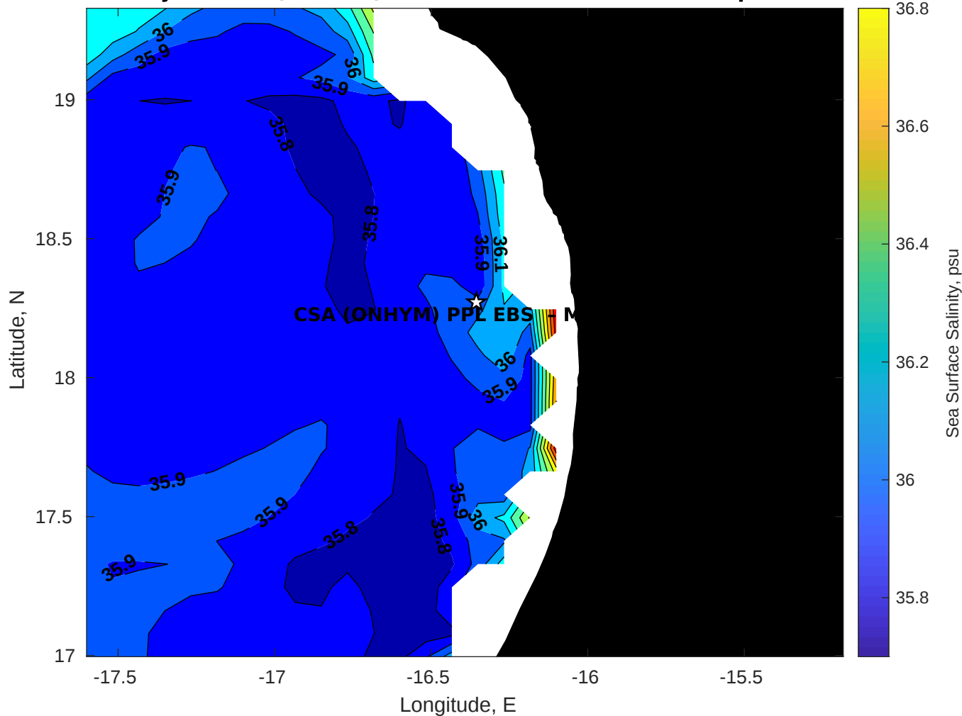
Surface Salinity for CSA (ONHYM) PPL EBS - Mauritania at 10-Apr-2025 00:00:00
