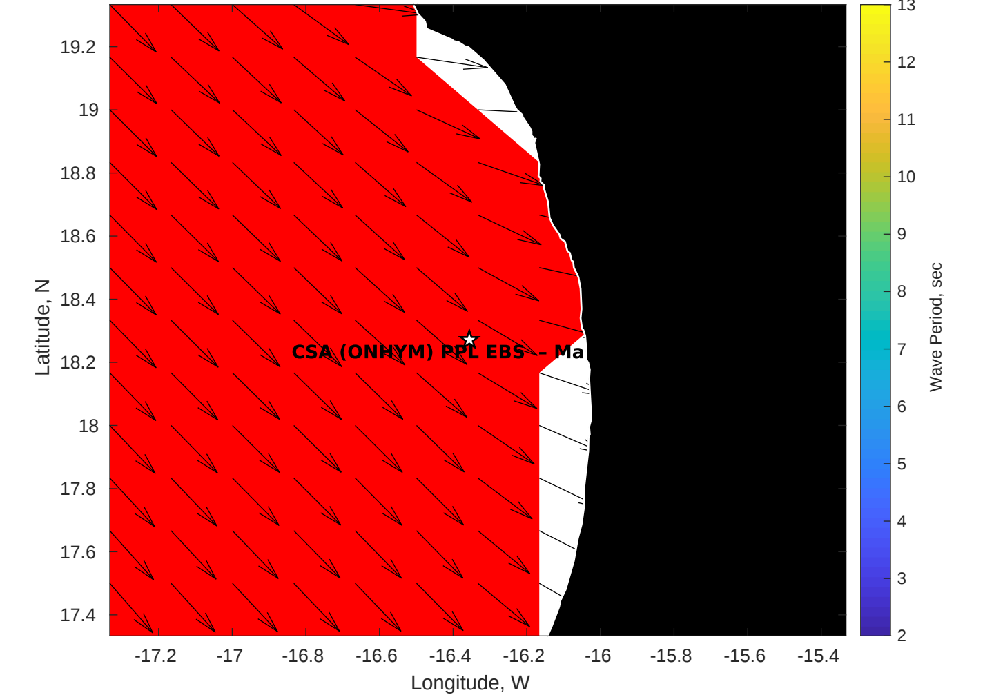
Wave Period (sec) for CSA (ONHYM) PPL EBS - Mauritania at 11-Apr-2025 09:00:00
