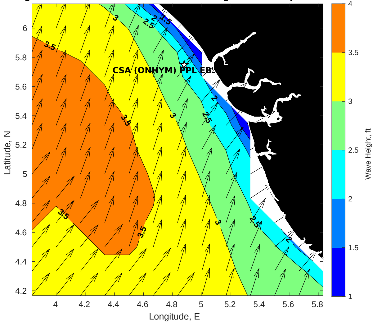
Wave Height (ft) for CSA (ONHYM) PPL EBS - Nigeria at 11-Apr-2025 09:00:00
