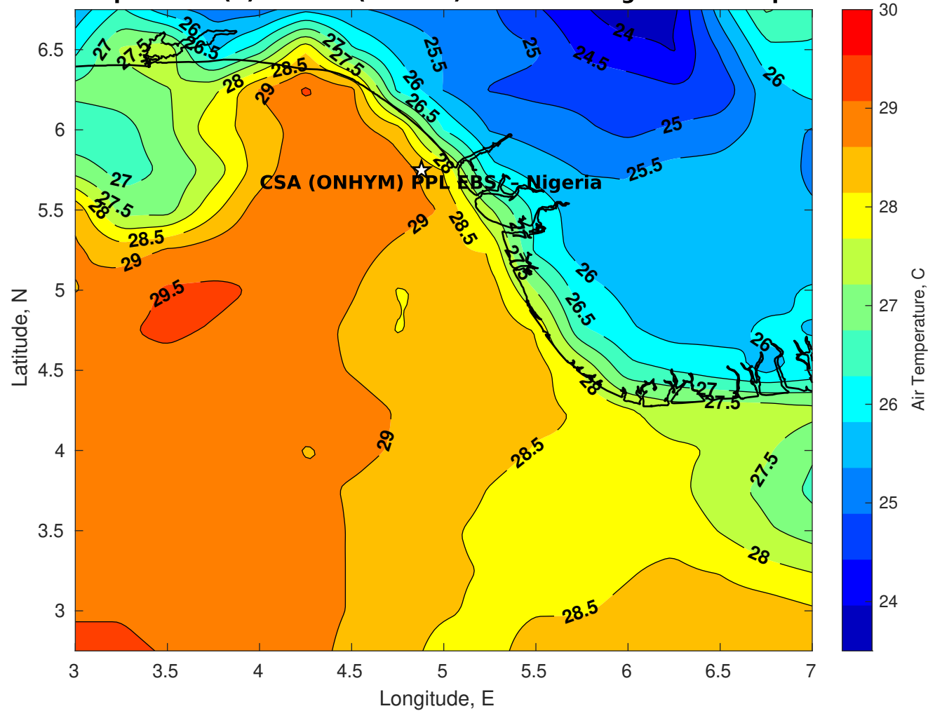
Air Temperature (C) for CSA (ONHYM) PPL EBS - Nigeria at 11-Apr-2025
