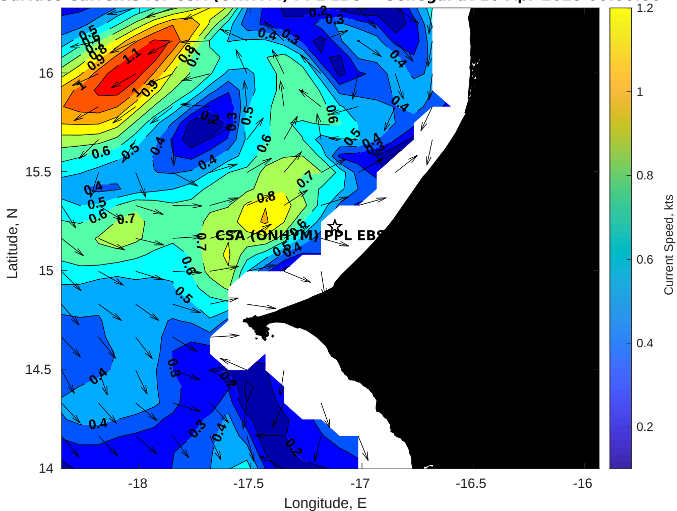
Surface Currents for CSA (ONHYM) PPL EBS - Senegal at 10-Apr-2025 00:00:00
