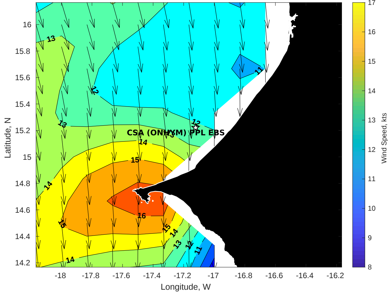
Winds (kts) for CSA (ONHYM) PPL EBS - Senegal at 11-Apr-2025 09:00:00
