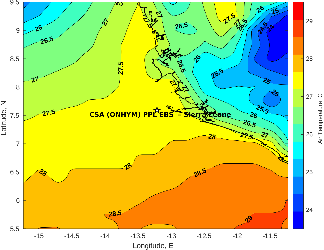
Air Temperature (C) for CSA (ONHYM) PPL EBS - Sierra Leone at 11-Apr-2025
