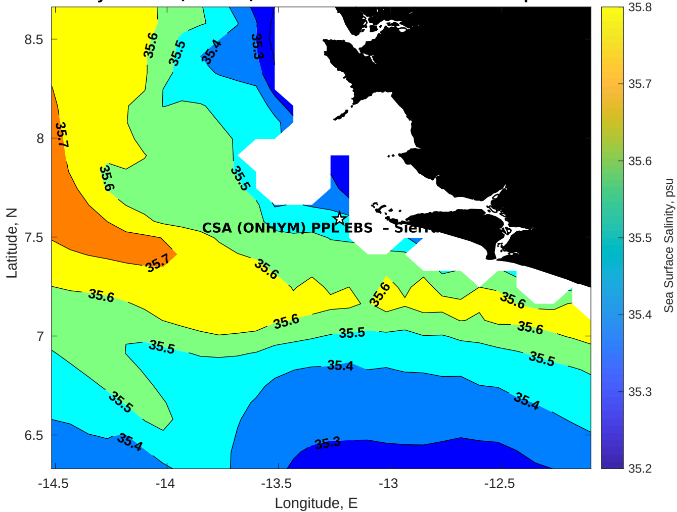
Surface Salinity for CSA (ONHYM) PPL EBS - Sierra Leone at 10-Apr-2025 00:00:00
