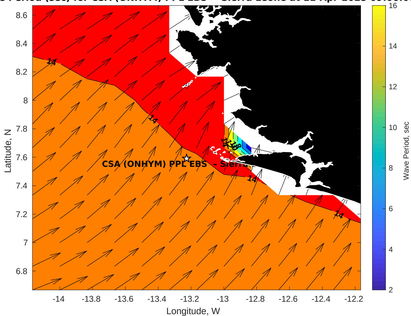
Wave Period (sec) for CSA (ONHYM) PPL EBS - Sierra Leone at 11-Apr-2025 09:00:00
