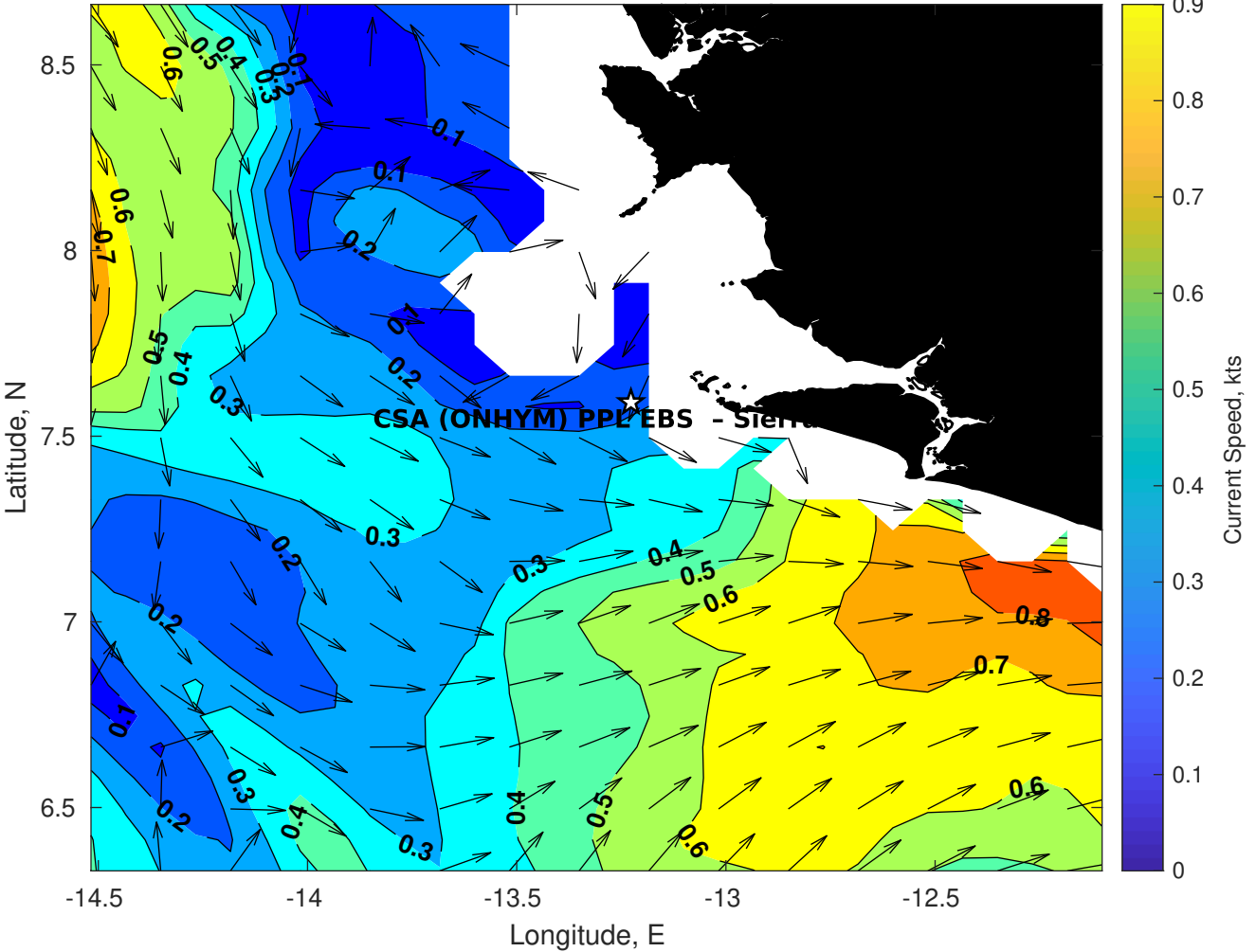
Surface Currents for CSA (ONHYM) PPL EBS - Sierra Leone at 10-Apr-2025 00:00:00
