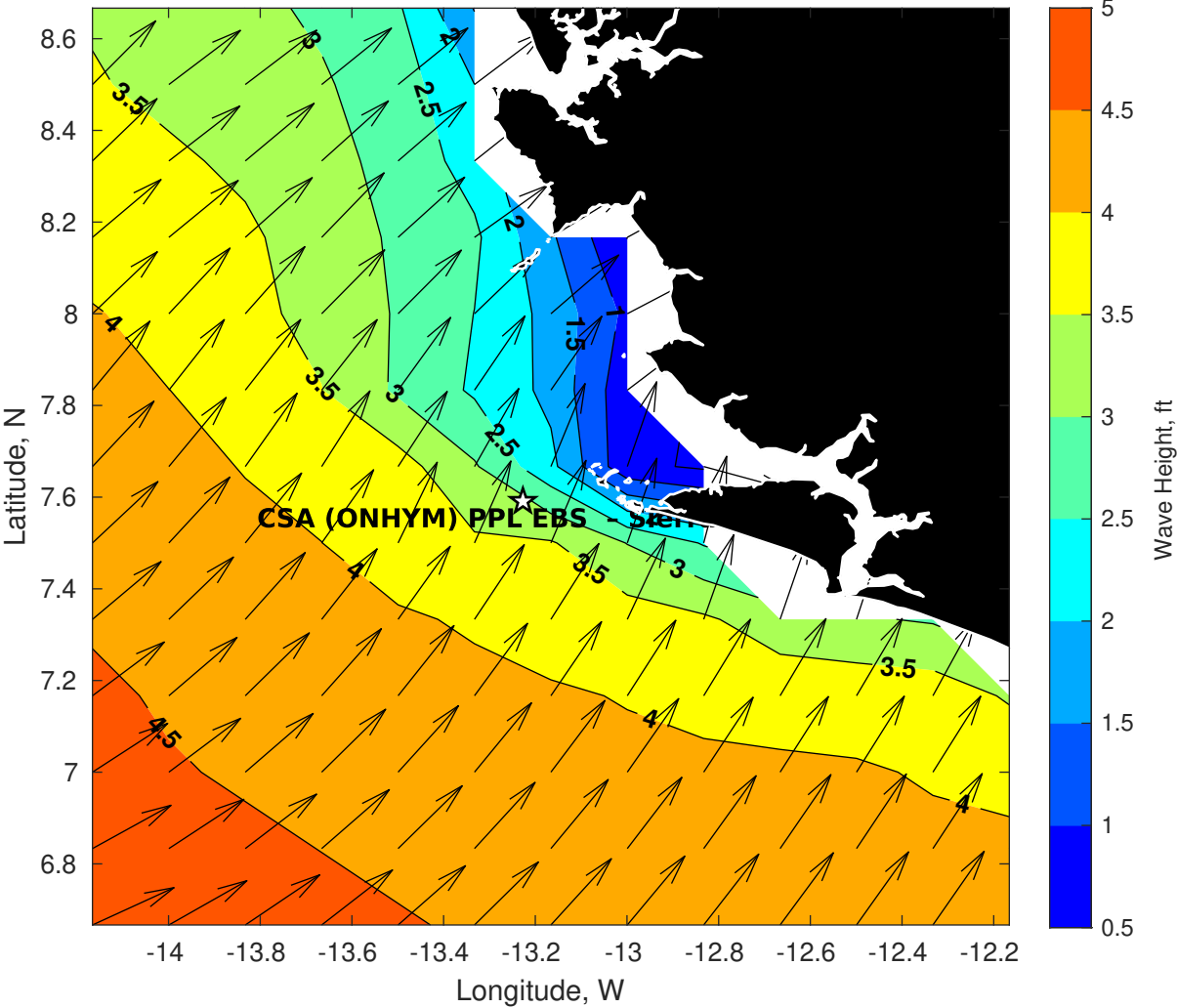
Wave Height (ft) for CSA (ONHYM) PPL EBS - Sierra Leone at 11-Apr-2025 09:00:00
