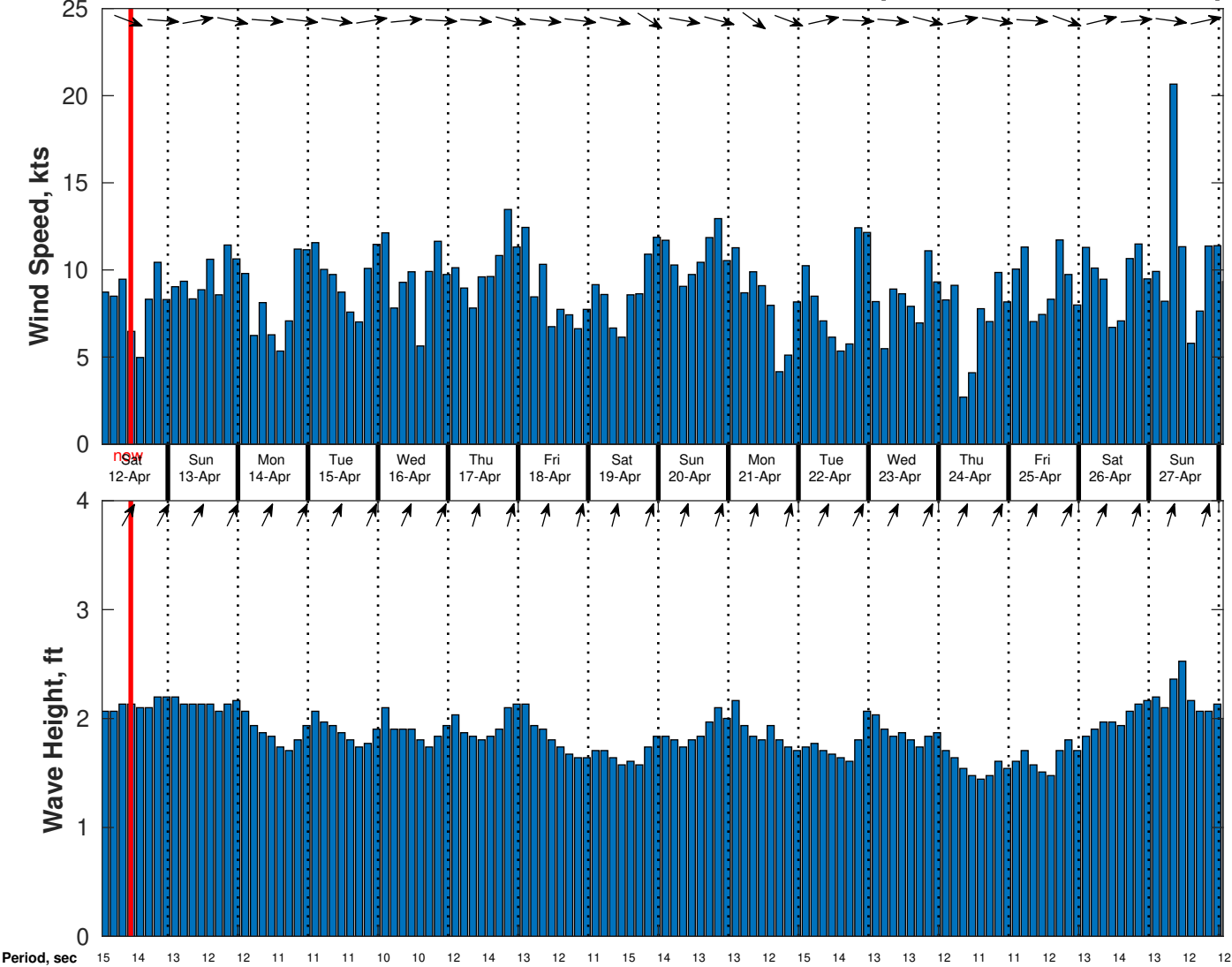
Wind & Wave Forecast for CSA (ONHYM) PPL EBS - Sierra Leone from 11-Apr-2025 01:00:00 to 27-Apr-2025 01:00:00
