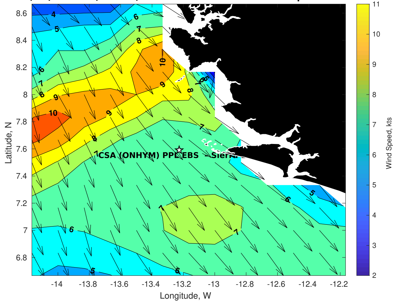
Winds (kts) for CSA (ONHYM) PPL EBS - Sierra Leone at 11-Apr-2025 09:00:00
