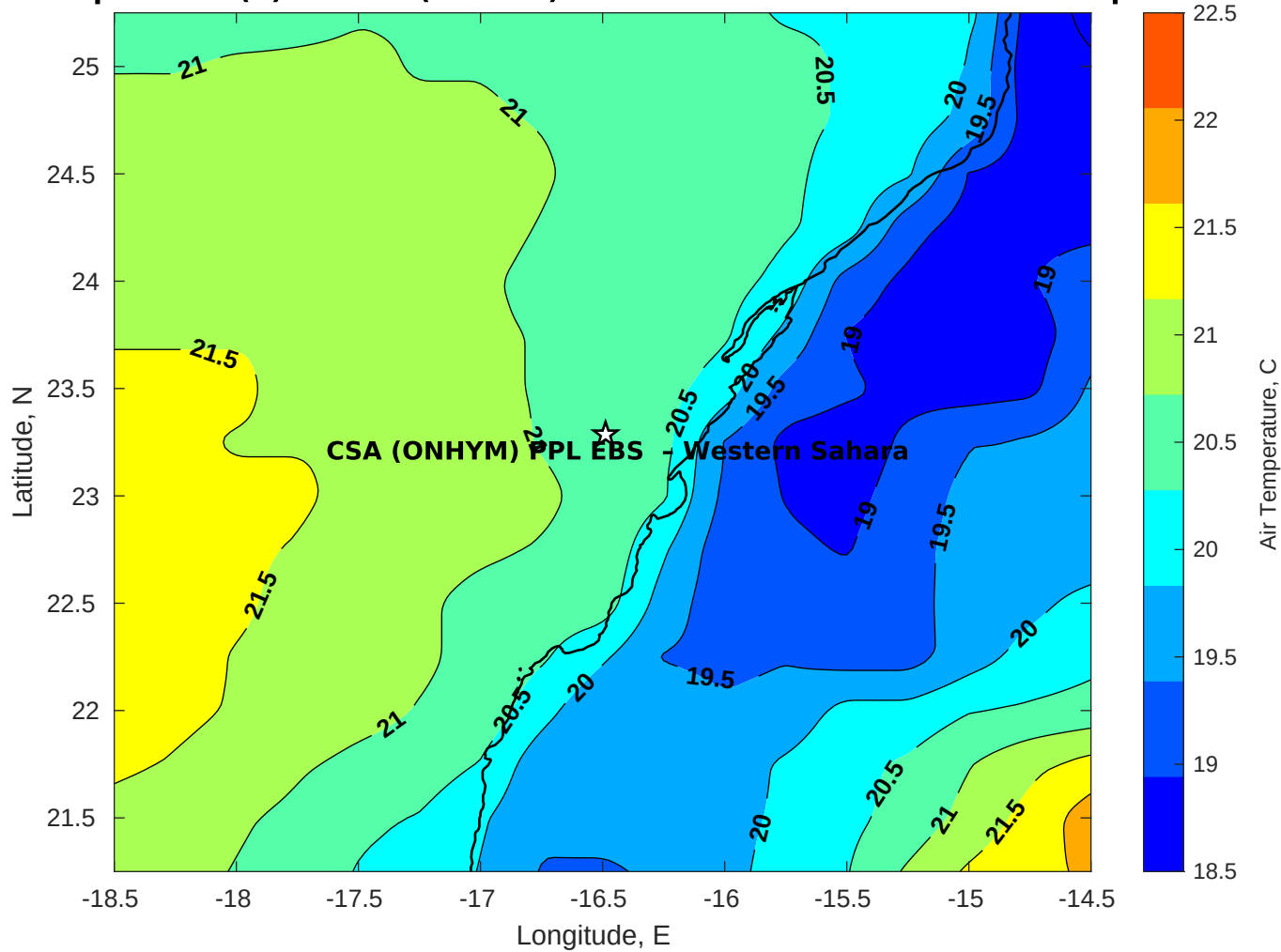
Air Temperature (C) for CSA (ONHYM) PPL EBS - Western Sahara at 11-Apr-2025
