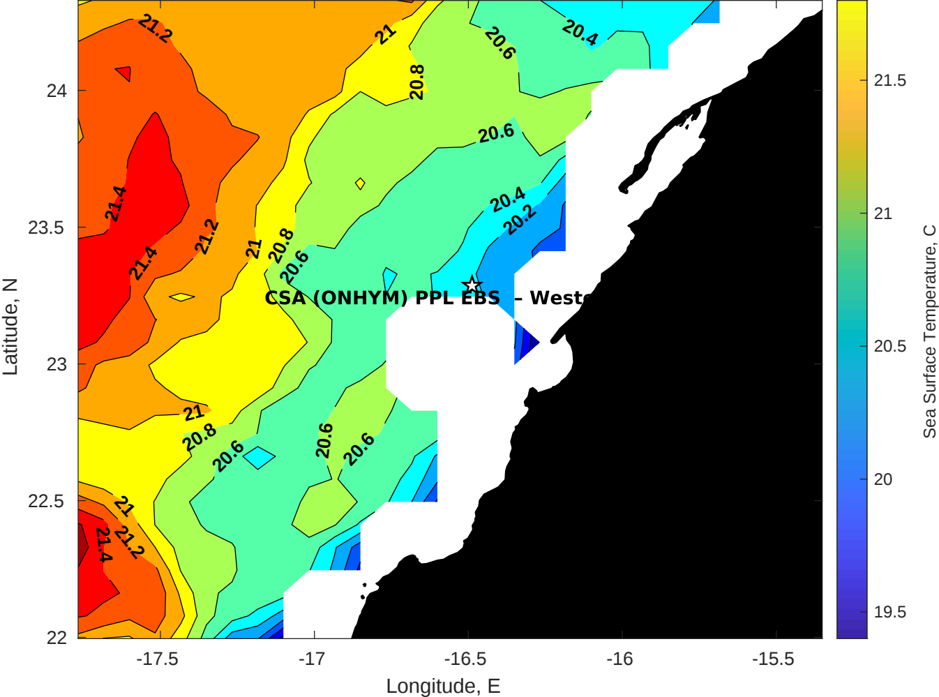
SST for CSA (ONHYM) PPL EBS - Western Sahara at 10-Apr-2025 00:00:00
