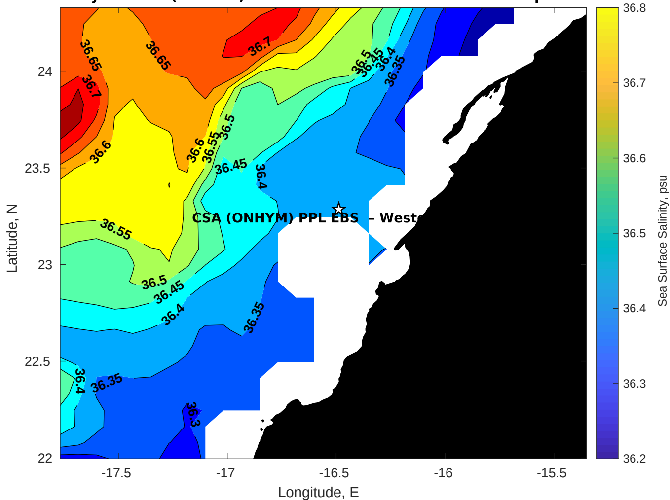
Surface Salinity for CSA (ONHYM) PPL EBS - Western Sahara at 10-Apr-2025 00:00:00
