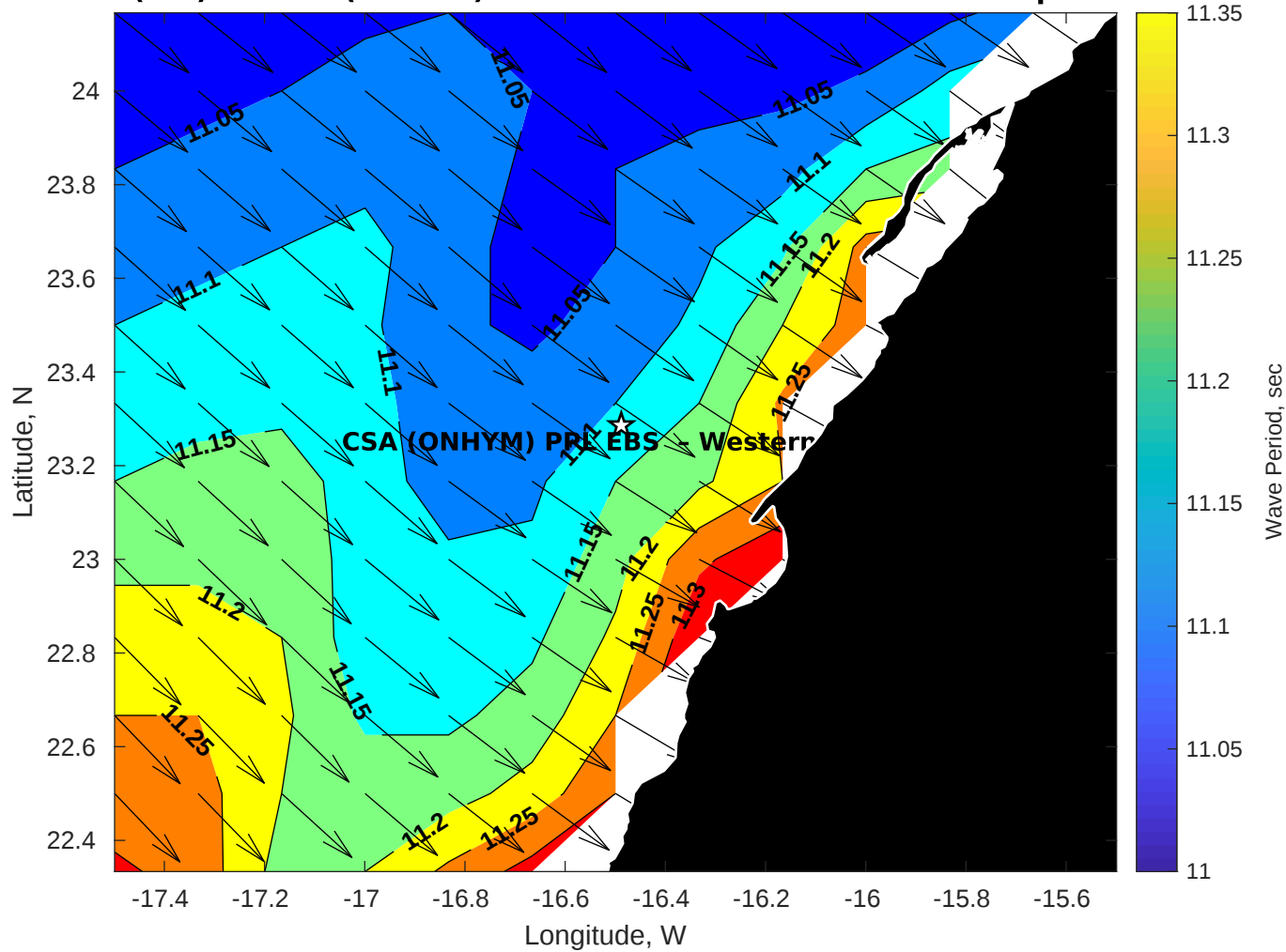
Wave Period (sec) for CSA (ONHYM) PPL EBS - Western Sahara at 11-Apr-2025 09:00:00
