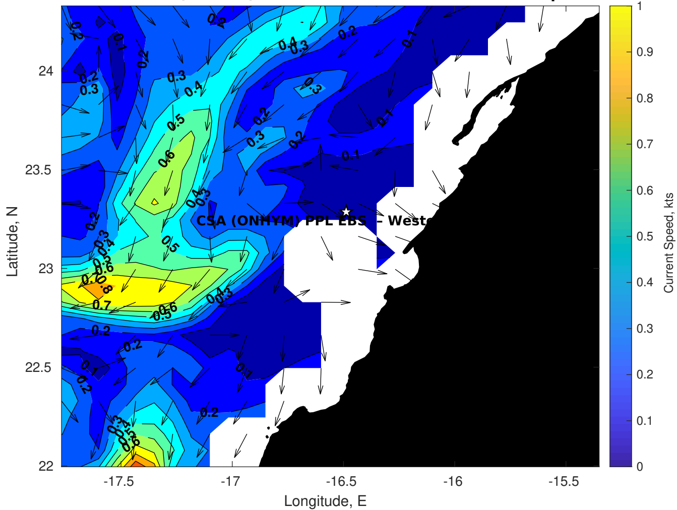
Surface Currents for CSA (ONHYM) PPL EBS - Western Sahara at 10-Apr-2025 00:00:00
