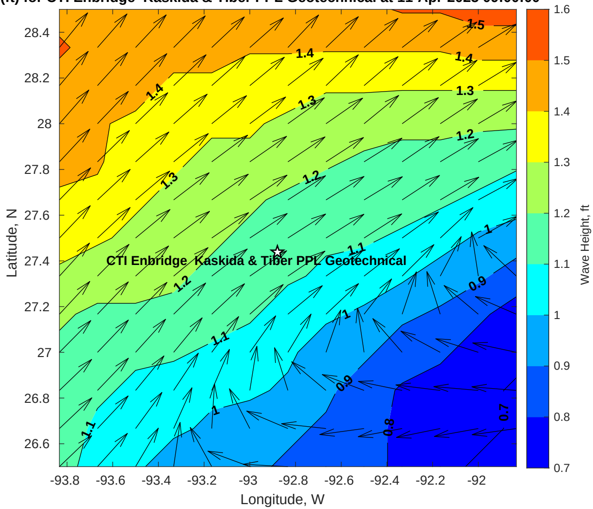
Wave Height (ft) for CTI Enbridge Kaskida & Tiber PPL Geotechnical at 11-Apr-2025 09:00:00
